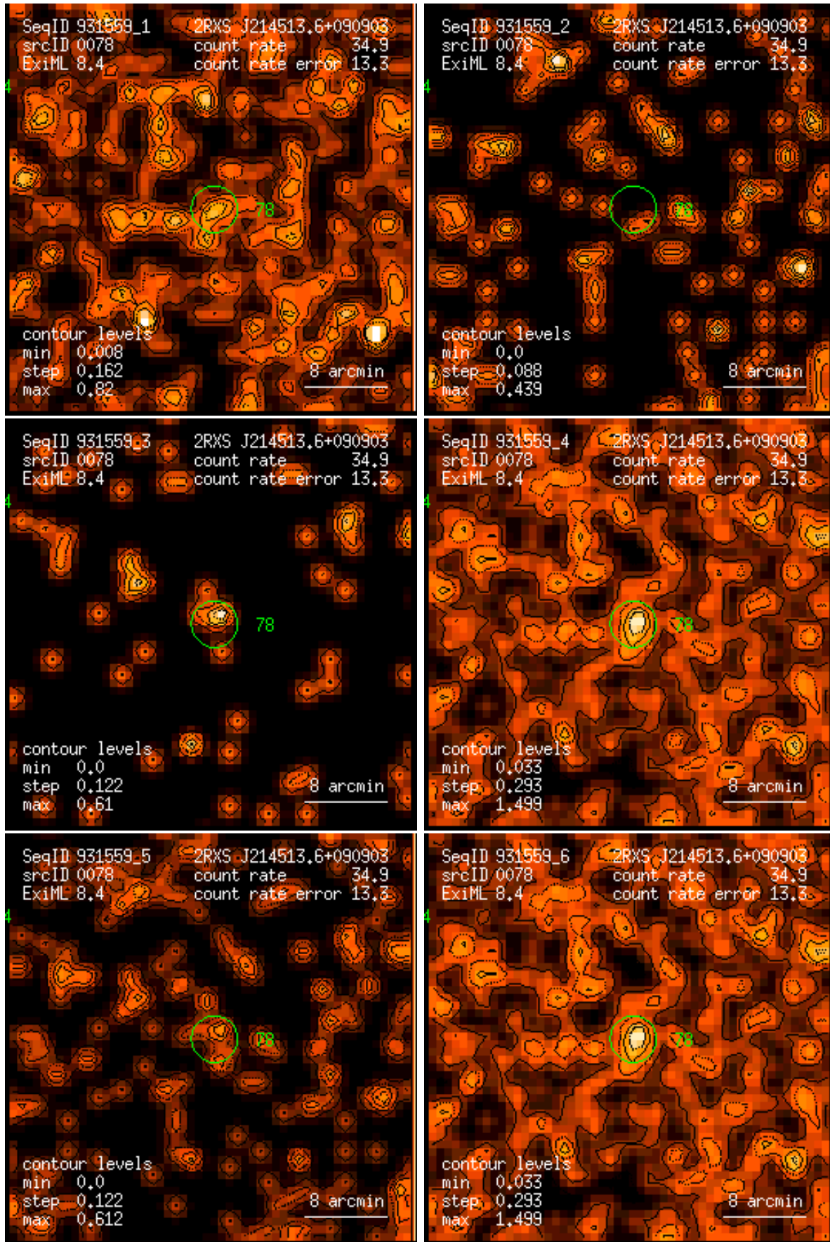
Figure 78: RASS 931559: detection 0078: band rate images, Gaussian filter: (1) PSPC channels 11 – 41, (2) 52 – 90, (3) 91 – 201, (4) 11 – 235, (5) 52 – 201, (6) 11 – 201. Broad band rates in counts/ks. Band rate contour levels in counts/ks/arcmin 2 .
