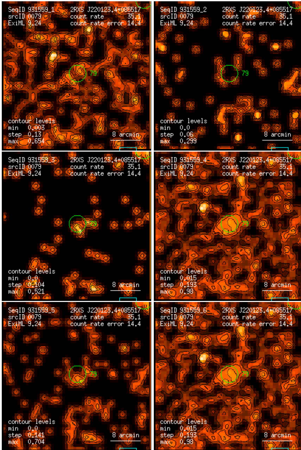
Figure 79: RASS 931559: detection 0079: band rate images, Gaussian filter: (1) PSPC channels 11 – 41, (2) 52 – 90, (3) 91 – 201, (4) 11 – 235, (5) 52 – 201, (6) 11 – 201. Broad band rates in counts/ks. Band rate contour levels in counts/ks/arcmin 2 .
