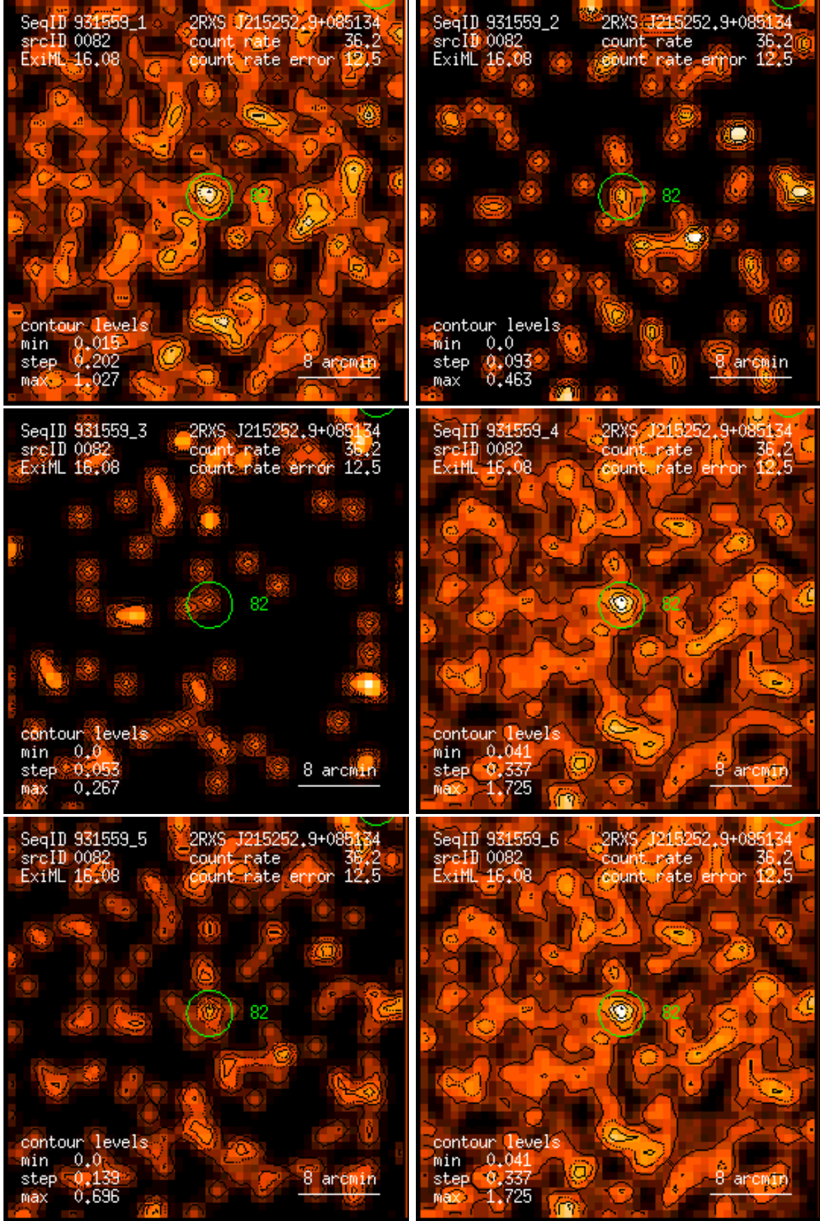
Figure 82: RASS 931559: detection 0082: band rate images, Gaussian filter: (1) PSPC channels 11 – 41, (2) 52 – 90, (3) 91 – 201, (4) 11 – 235, (5) 52 – 201, (6) 11 – 201. Broad band rates in counts/ks. Band rate contour levels in counts/ks/arcmin 2 .
