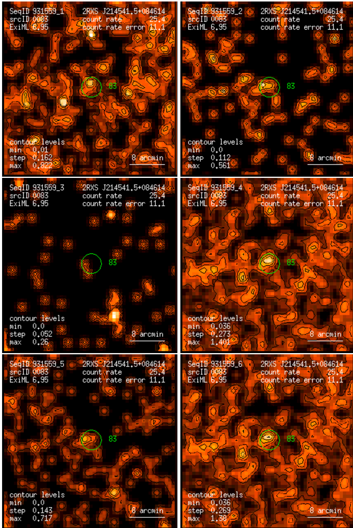
Figure 83: RASS 931559: detection 0083: band rate images, Gaussian filter: (1) PSPC channels 11 – 41, (2) 52 – 90, (3) 91 – 201, (4) 11 – 235, (5) 52 – 201, (6) 11 – 201. Broad band rates in counts/ks. Band rate contour levels in counts/ks/arcmin 2 .
