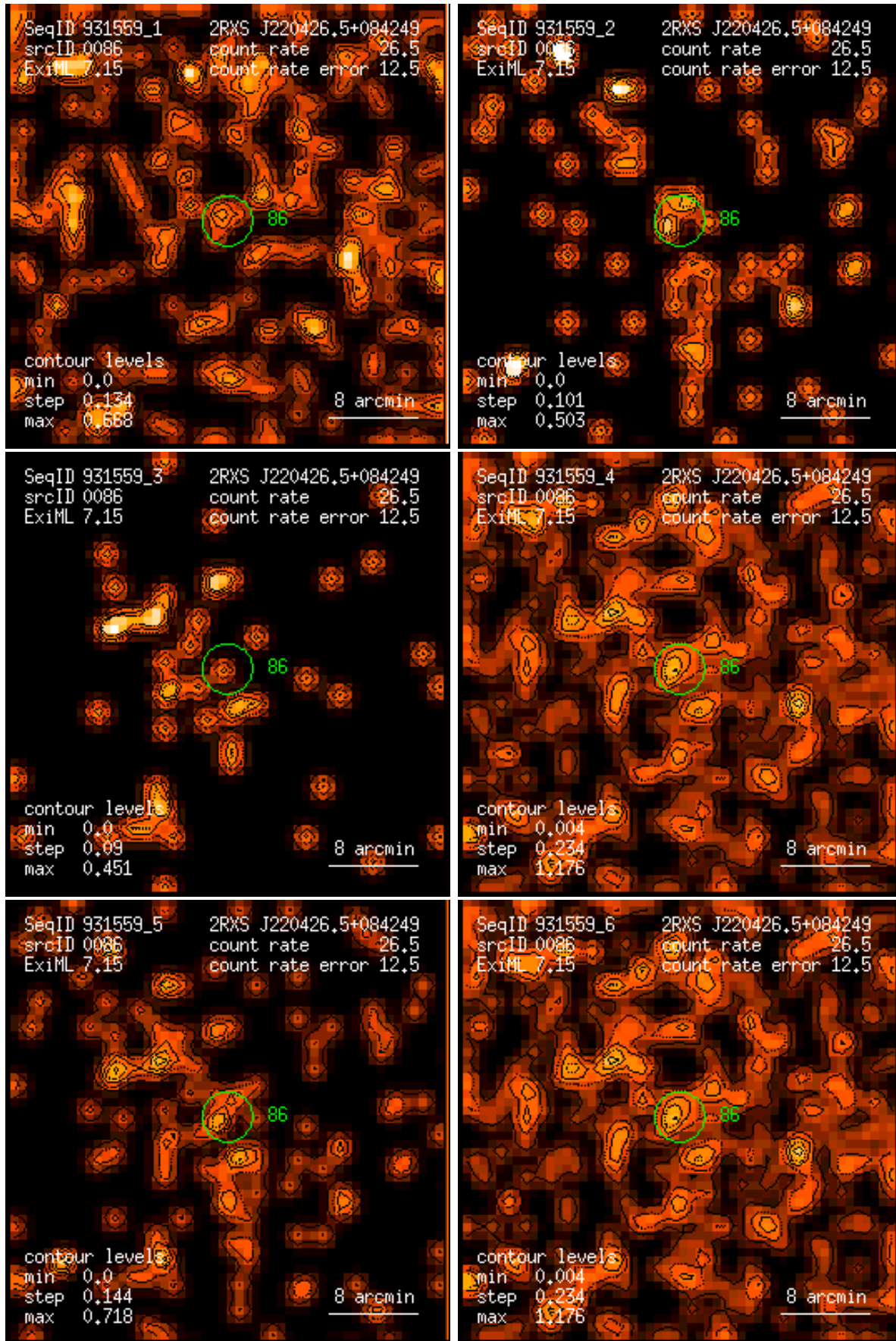
Figure 86: RASS 931559: detection 0086: band rate images, Gaussian filter: (1) PSPC channels 11 – 41, (2) 52 – 90, (3) 91 – 201, (4) 11 – 235, (5) 52 – 201, (6) 11 – 201. Broad band rates in counts/ks. Band rate contour levels in counts/ks/arcmin 2 .
