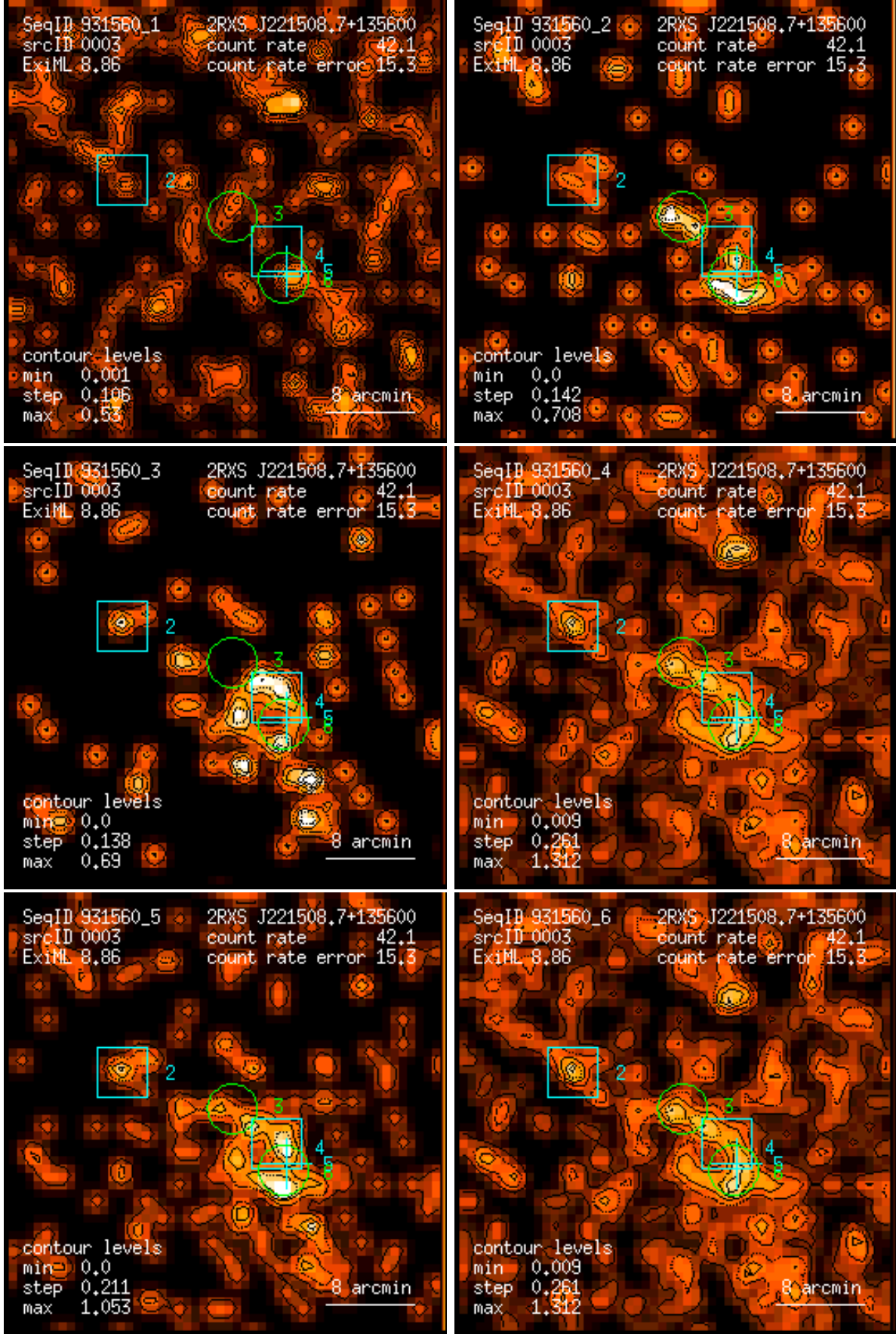
Figure 3: RASS 931560: detection 0003: band rate images, Gaussian filter: (1) PSPC channels 11 – 41, (2) 52 – 90, (3) 91 – 201, (4) 11 – 235, (5) 52 – 201, (6) 11 – 201. Broad band rates in counts/ks. Band rate contour levels in counts/ks/arcmin 2 .
