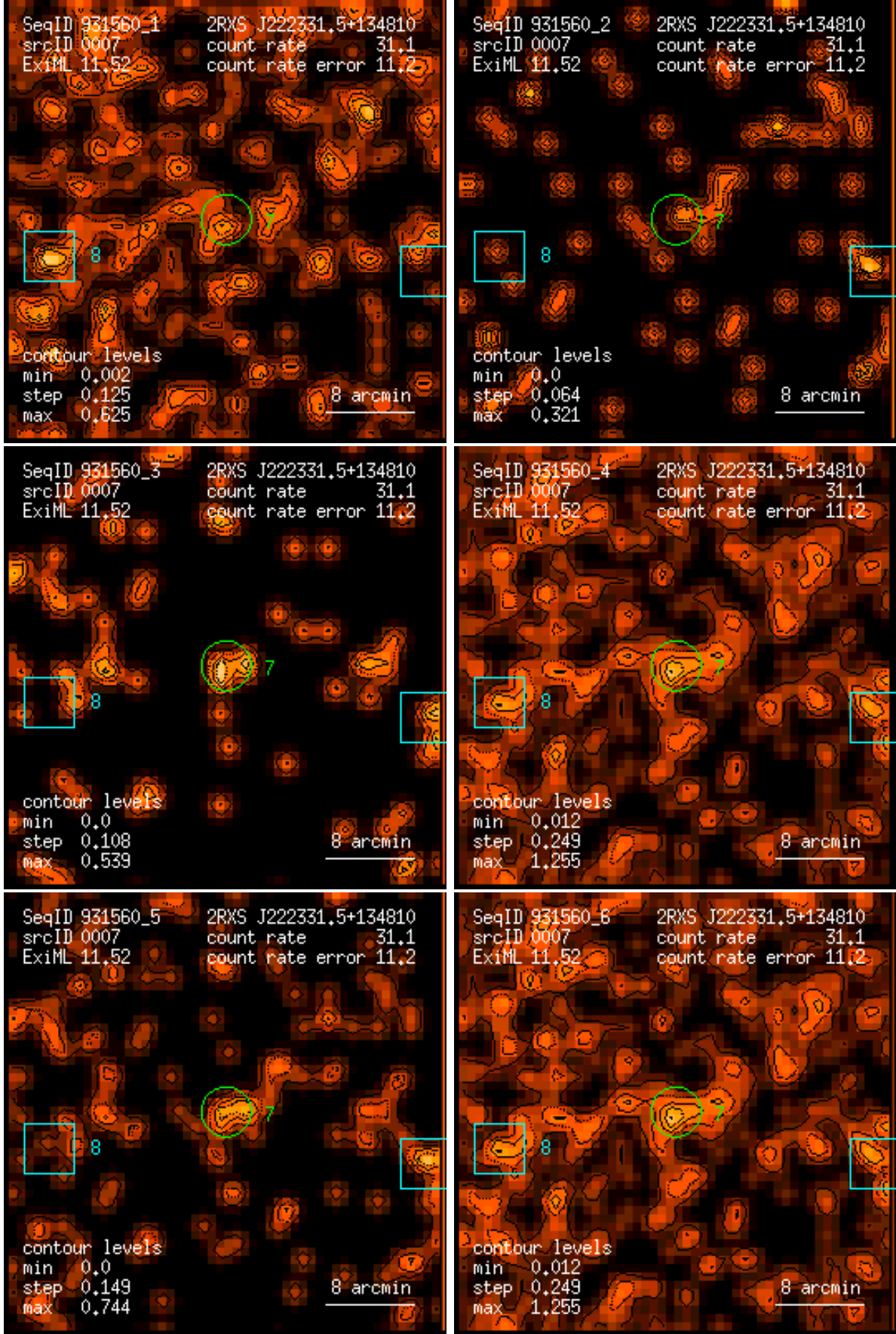
Figure 7: RASS 931560: detection 0007: band rate images, Gaussian filter: (1) PSPC channels 11 – 41, (2) 52 – 90, (3) 91 – 201, (4) 11 – 235, (5) 52 – 201, (6) 11 – 201. Broad band rates in counts/ks. Band rate contour levels in counts/ks/arcmin 2 .
