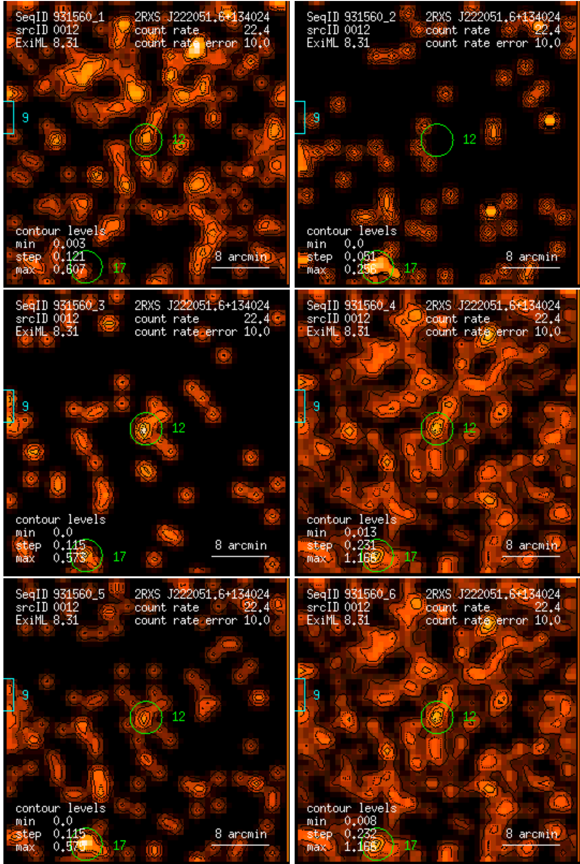
Figure 12: RASS 931560: detection 0012: band rate images, Gaussian filter: (1) PSPC channels 11 – 41, (2) 52 – 90, (3) 91 – 201, (4) 11 – 235, (5) 52 – 201, (6) 11 – 201. Broad band rates in counts/ks. Band rate contour levels in counts/ks/arcmin 2 .
