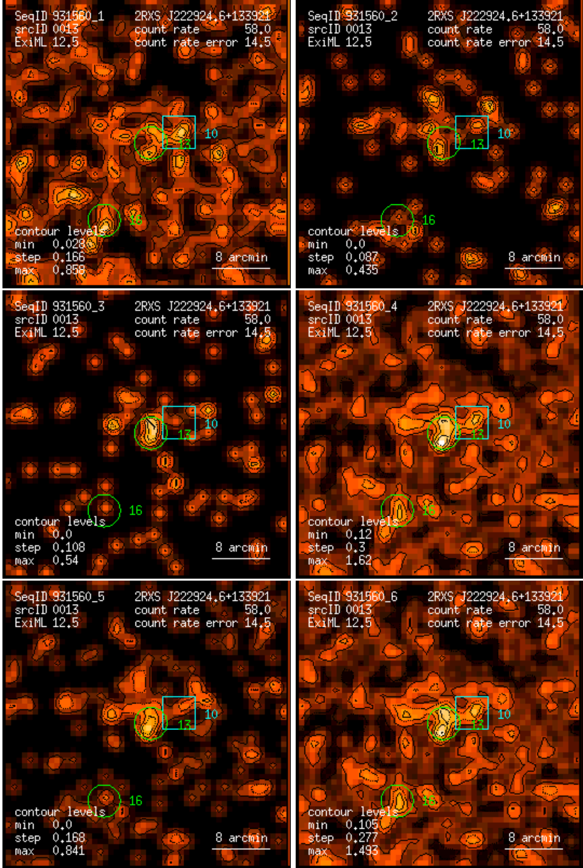
Figure 13: RASS 931560: detection 0013: band rate images, Gaussian filter: (1) PSPC channels 11 – 41, (2) 52 – 90, (3) 91 – 201, (4) 11 – 235, (5) 52 – 201, (6) 11 – 201. Broad band rates in counts/ks. Band rate contour levels in counts/ks/arcmin 2 .
