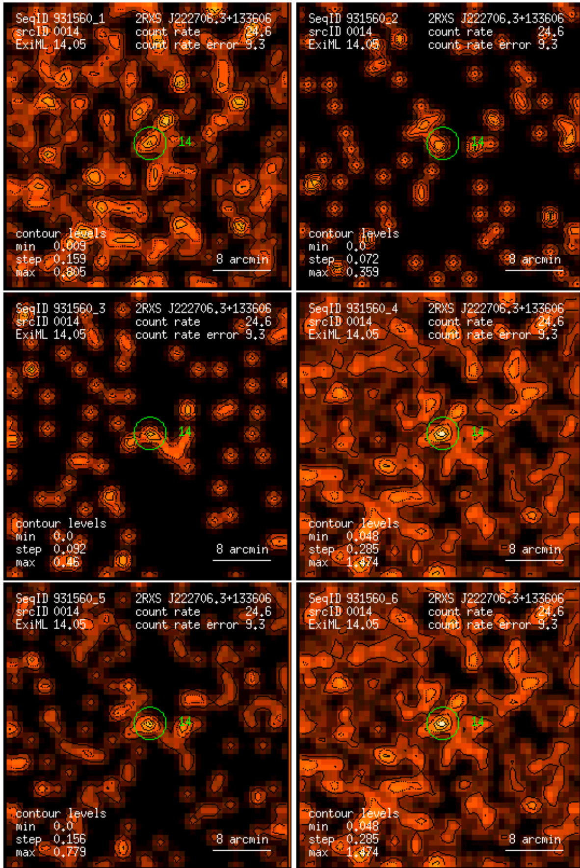
Figure 14: RASS 931560: detection 0014: band rate images, Gaussian filter: (1) PSPC channels 11 – 41, (2) 52 – 90, (3) 91 – 201, (4) 11 – 235, (5) 52 – 201, (6) 11 – 201. Broad band rates in counts/ks. Band rate contour levels in counts/ks/arcmin 2 .
