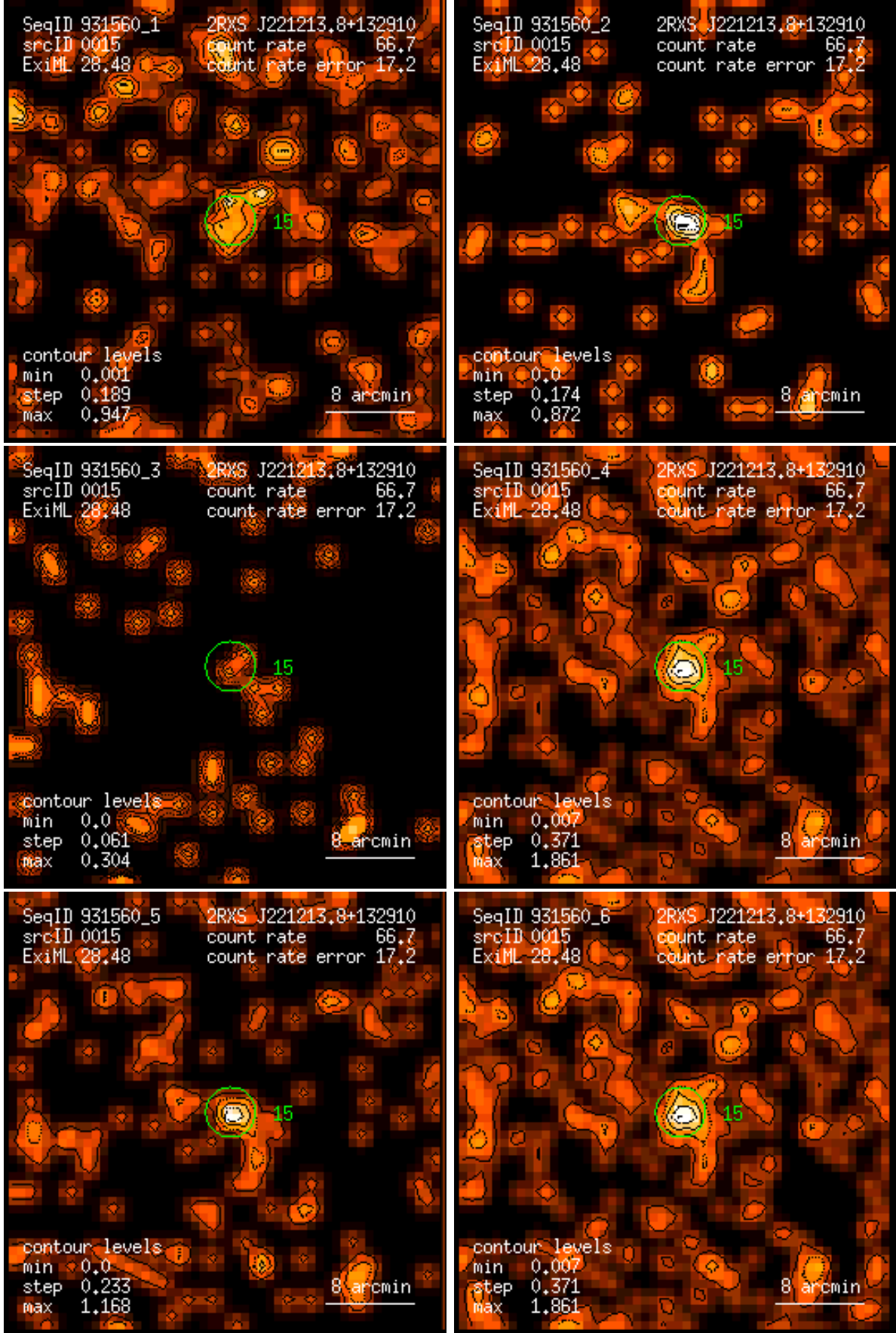
Figure 15: RASS 931560: detection 0015: band rate images, Gaussian filter: (1) PSPC channels 11 – 41, (2) 52 – 90, (3) 91 – 201, (4) 11 – 235, (5) 52 – 201, (6) 11 – 201. Broad band rates in counts/ks. Band rate contour levels in counts/ks/arcmin 2 .
