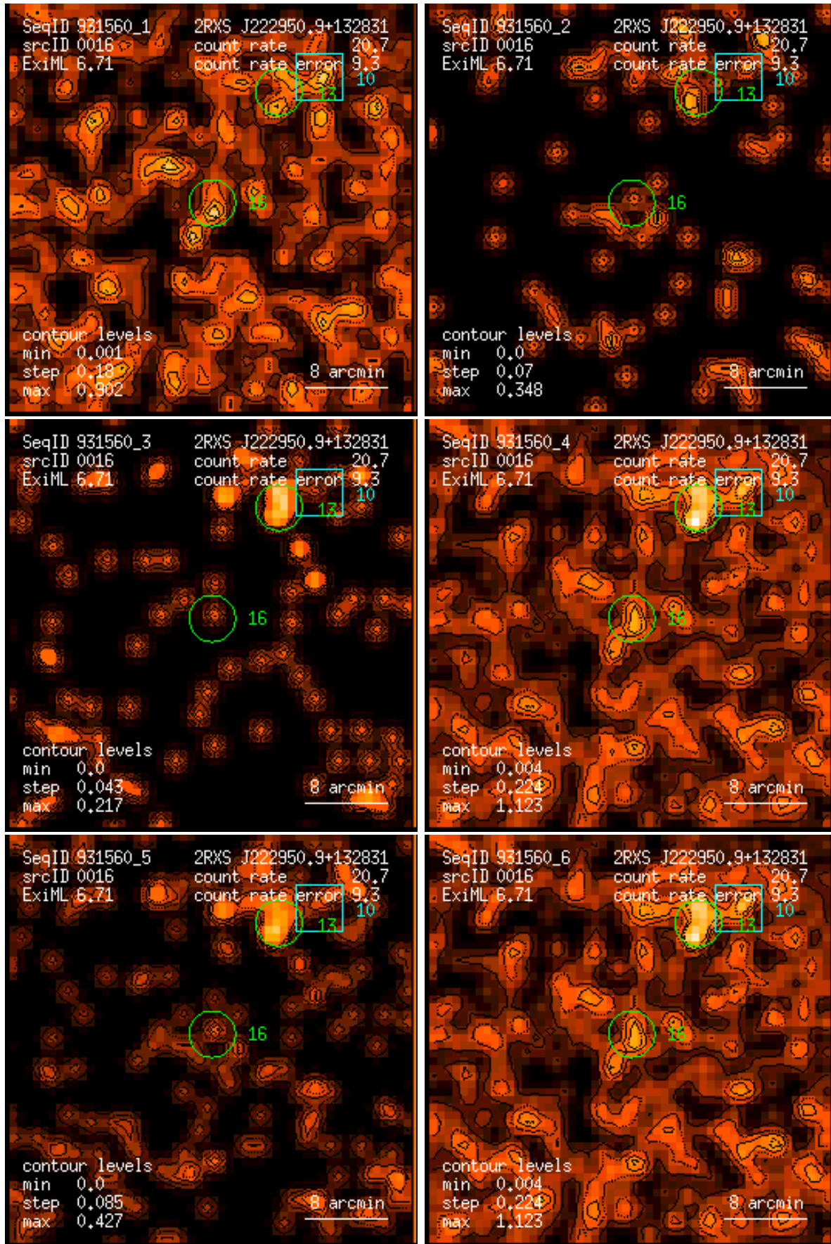
Figure 16: RASS 931560: detection 0016: band rate images, Gaussian filter: (1) PSPC channels 11 – 41, (2) 52 – 90, (3) 91 – 201, (4) 11 – 235, (5) 52 – 201, (6) 11 – 201. Broad band rates in counts/ks. Band rate contour levels in counts/ks/arcmin 2 .
