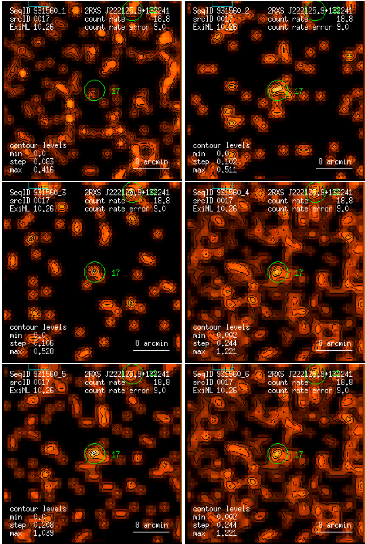
Figure 17: RASS 931560: detection 0017: band rate images, Gaussian filter: (1) PSPC channels 11 – 41, (2) 52 – 90, (3) 91 – 201, (4) 11 – 235, (5) 52 – 201, (6) 11 – 201. Broad band rates in counts/ks. Band rate contour levels in counts/ks/arcmin 2 .
