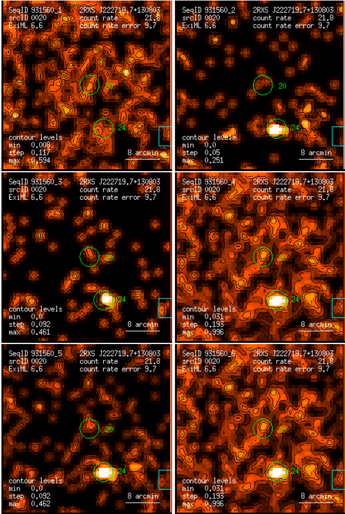
Figure 20: RASS 931560: detection 0020: band rate images, Gaussian filter: (1) PSPC channels 11 – 41, (2) 52 – 90, (3) 91 – 201, (4) 11 – 235, (5) 52 – 201, (6) 11 – 201. Broad band rates in counts/ks. Band rate contour levels in counts/ks/arcmin 2 .
