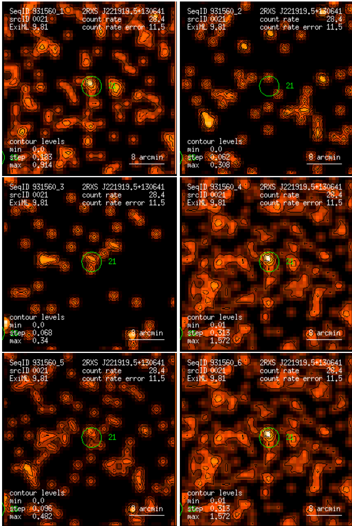
Figure 21: RASS 931560: detection 0021: band rate images, Gaussian filter: (1) PSPC channels 11 – 41, (2) 52 – 90, (3) 91 – 201, (4) 11 – 235, (5) 52 – 201, (6) 11 – 201. Broad band rates in counts/ks. Band rate contour levels in counts/ks/arcmin 2 .
