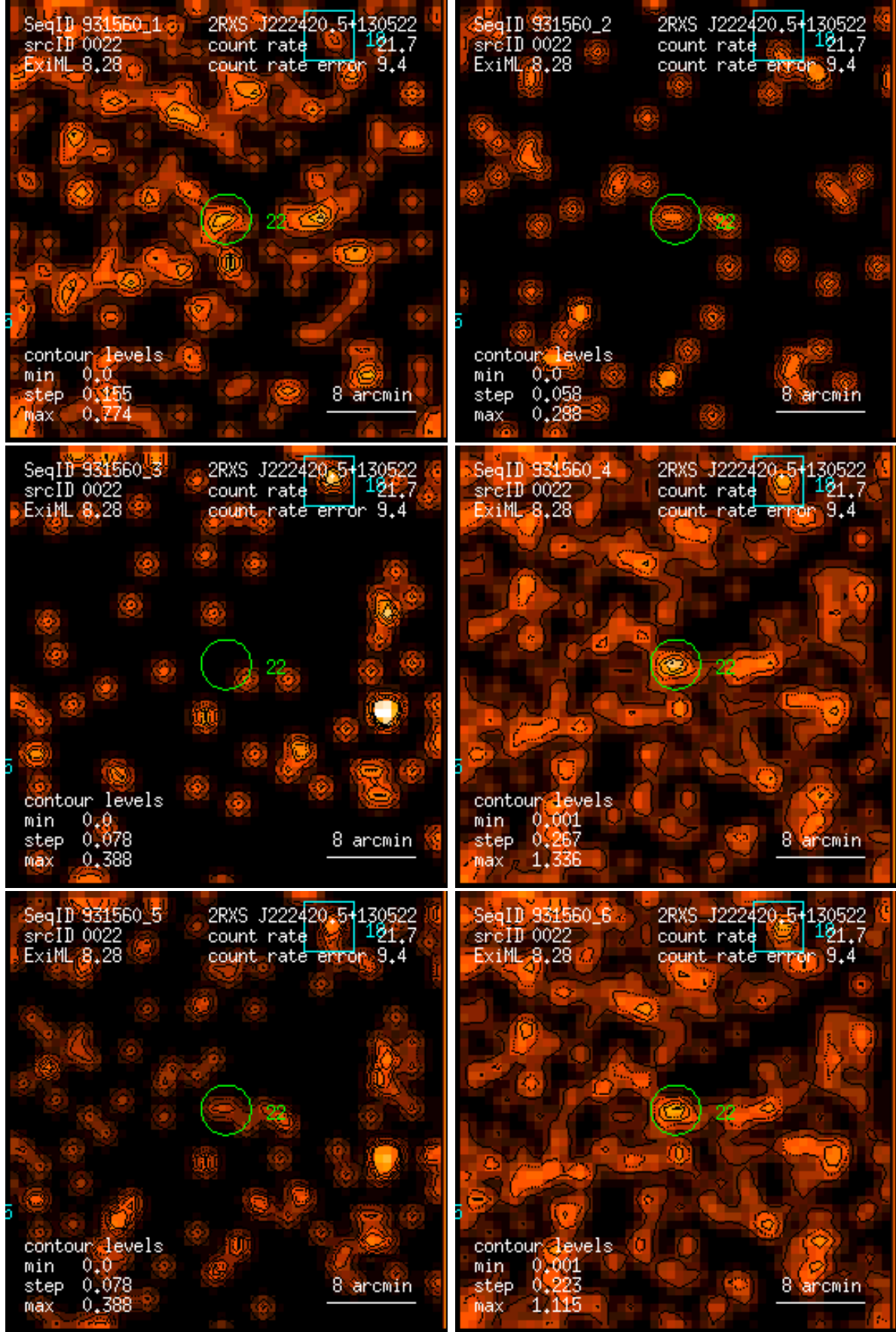
Figure 22: RASS 931560: detection 0022: band rate images, Gaussian filter: (1) PSPC channels 11 – 41, (2) 52 – 90, (3) 91 – 201, (4) 11 – 235, (5) 52 – 201, (6) 11 – 201. Broad band rates in counts/ks. Band rate contour levels in counts/ks/arcmin 2 .
