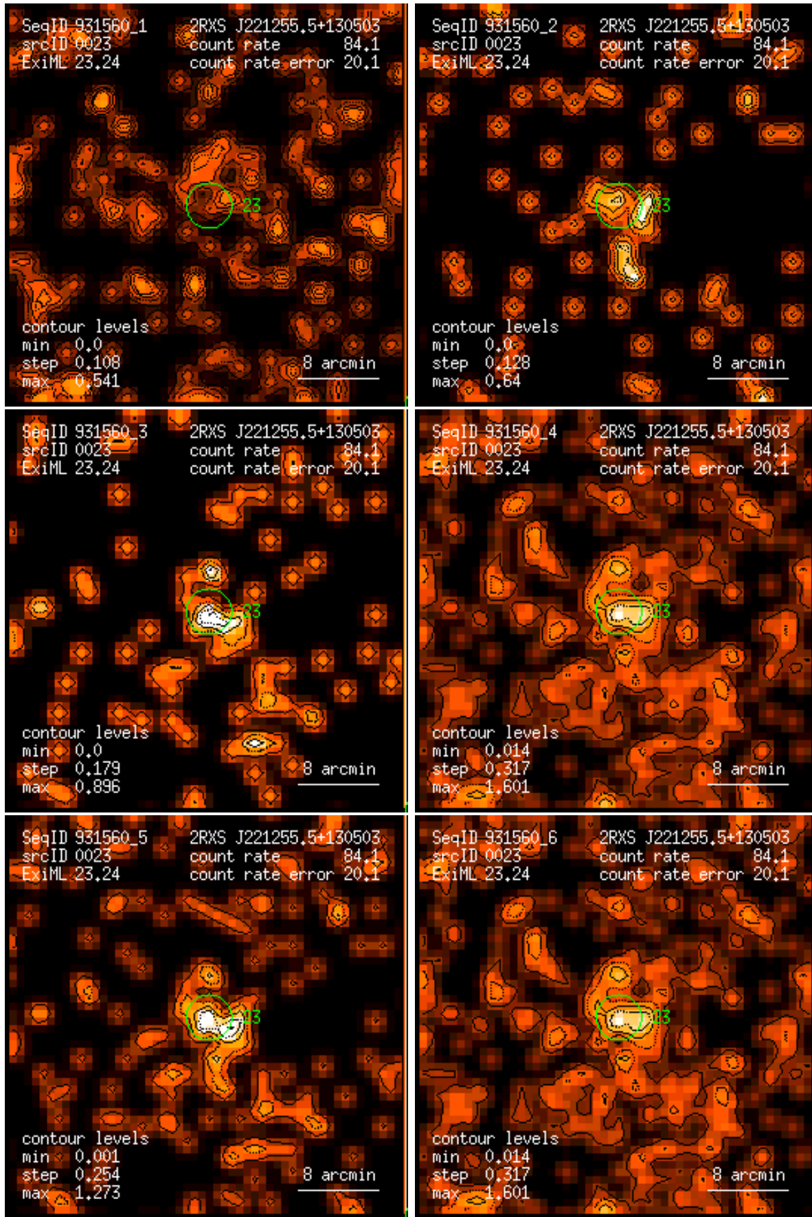
Figure 23: RASS 931560: detection 0023: band rate images, Gaussian filter: (1) PSPC channels 11 – 41, (2) 52 – 90, (3) 91 – 201, (4) 11 – 235, (5) 52 – 201, (6) 11 – 201. Broad band rates in counts/ks. Band rate contour levels in counts/ks/arcmin 2 .
