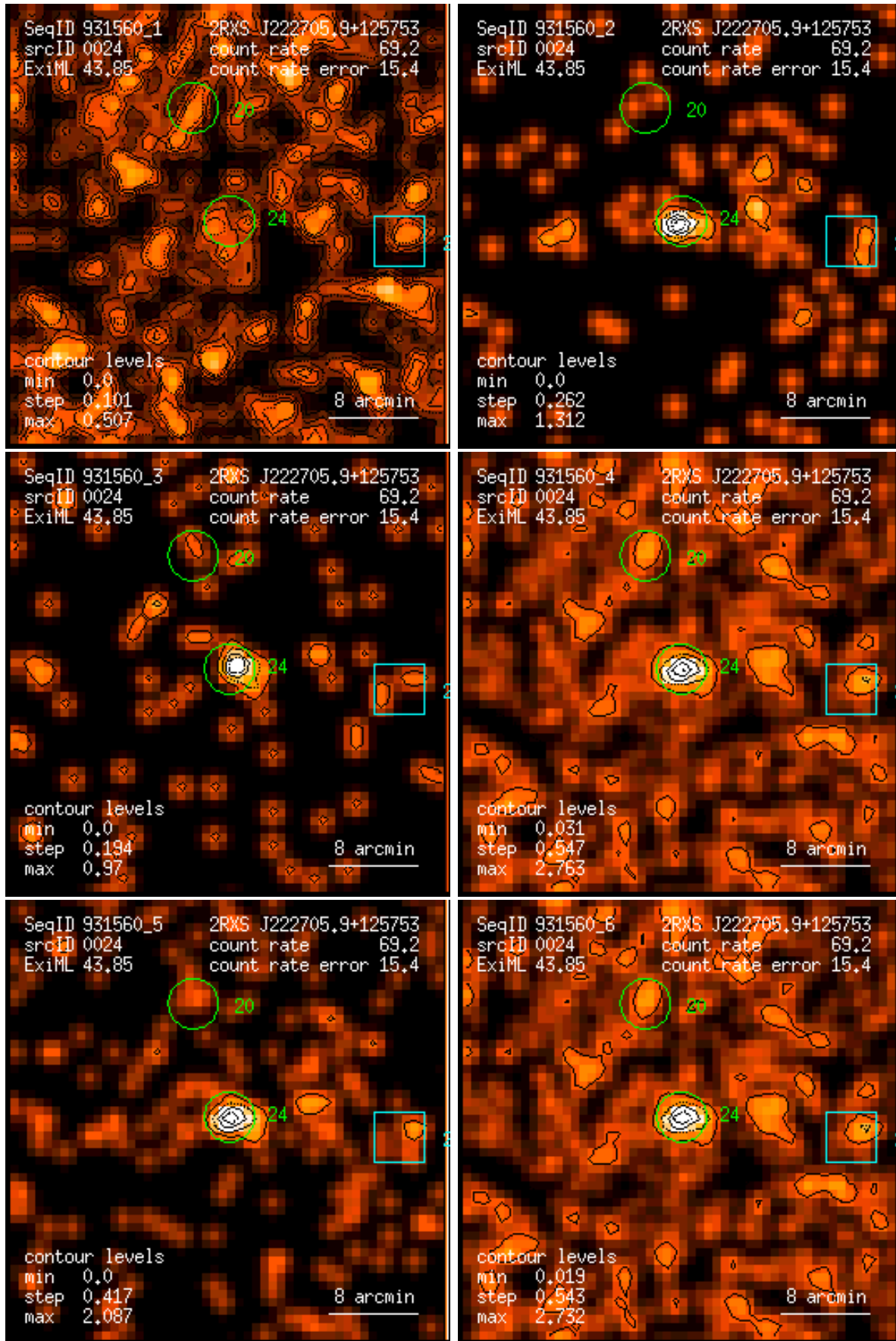
Figure 24: RASS 931560: detection 0024: band rate images, Gaussian filter: (1) PSPC channels 11 – 41, (2) 52 – 90, (3) 91 – 201, (4) 11 – 235, (5) 52 – 201, (6) 11 – 201. Broad band rates in counts/ks. Band rate contour levels in counts/ks/arcmin 2 .
