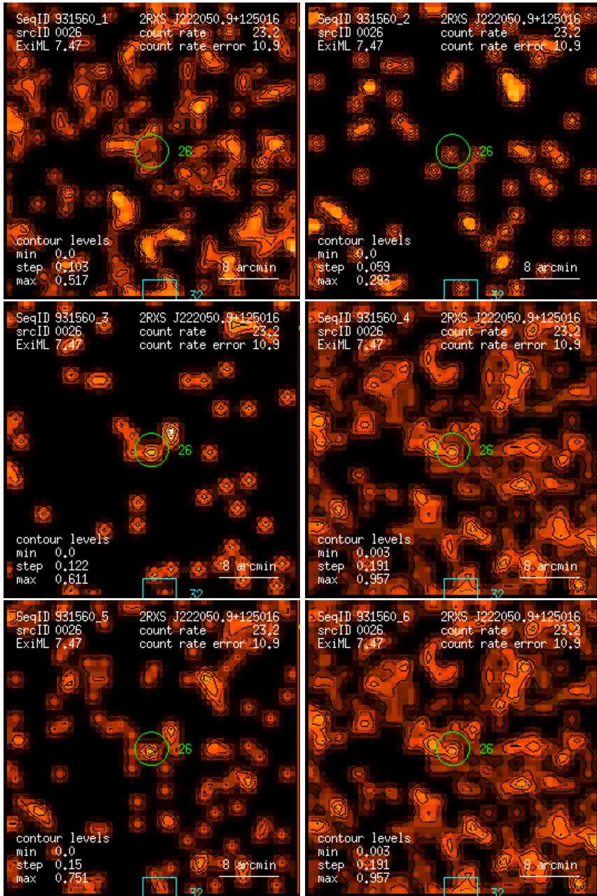
Figure 26: RASS 931560: detection 0026: band rate images, Gaussian filter: (1) PSPC channels 11 – 41, (2) 52 – 90, (3) 91 – 201, (4) 11 – 235, (5) 52 – 201, (6) 11 – 201. Broad band rates in counts/ks. Band rate contour levels in counts/ks/arcmin 2 .
