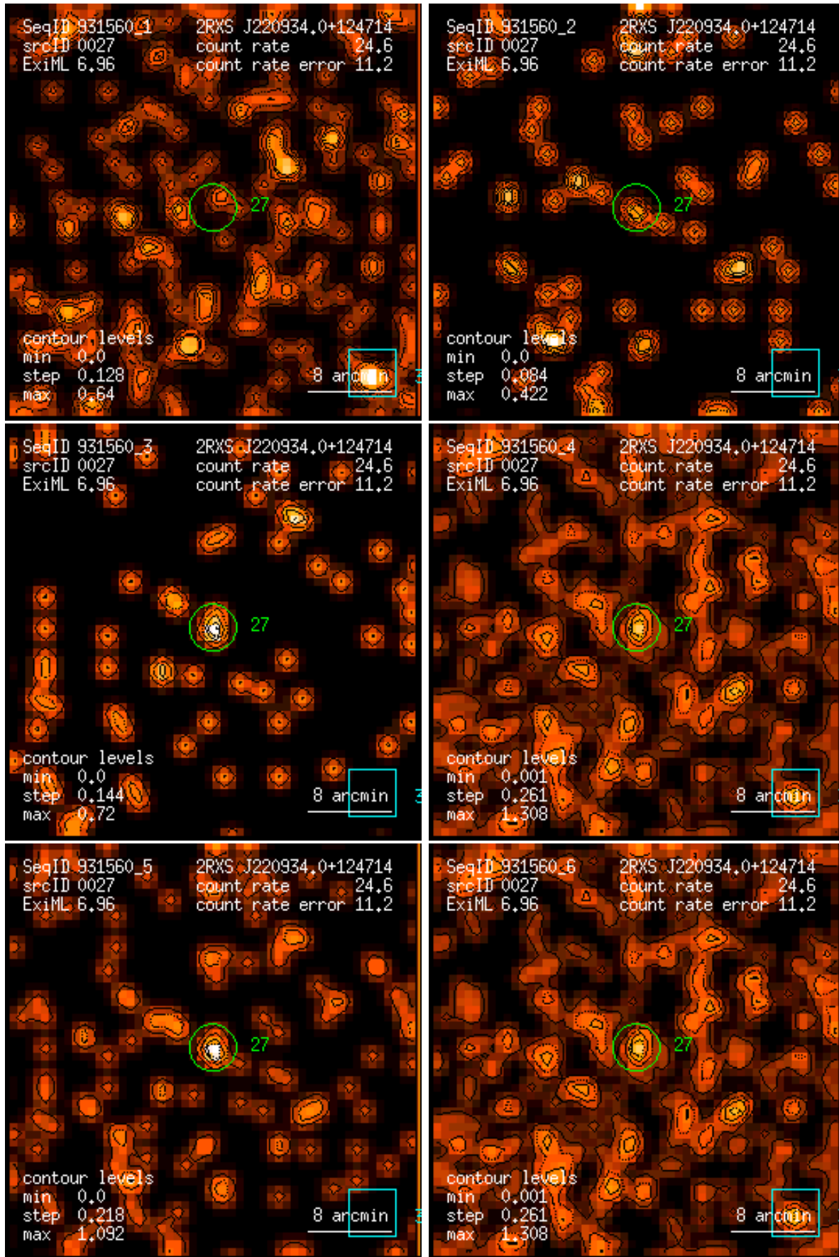
Figure 27: RASS 931560: detection 0027: band rate images, Gaussian filter: (1) PSPC channels 11 – 41, (2) 52 – 90, (3) 91 – 201, (4) 11 – 235, (5) 52 – 201, (6) 11 – 201. Broad band rates in counts/ks. Band rate contour levels in counts/ks/arcmin 2 .
