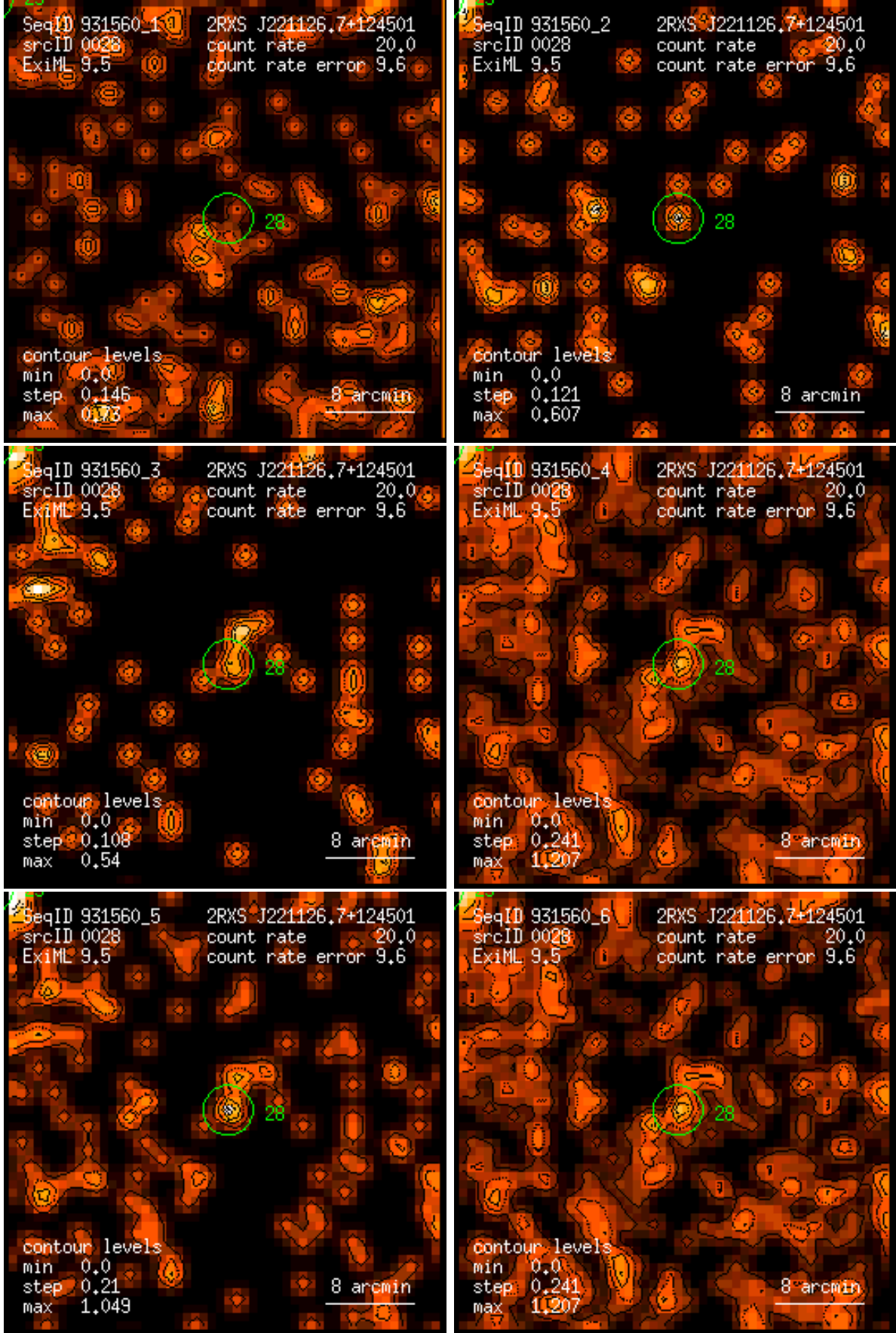
Figure 28: RASS 931560: detection 0028: band rate images, Gaussian filter: (1) PSPC channels 11 – 41, (2) 52 – 90, (3) 91 – 201, (4) 11 – 235, (5) 52 – 201, (6) 11 – 201. Broad band rates in counts/ks. Band rate contour levels in counts/ks/arcmin 2 .
