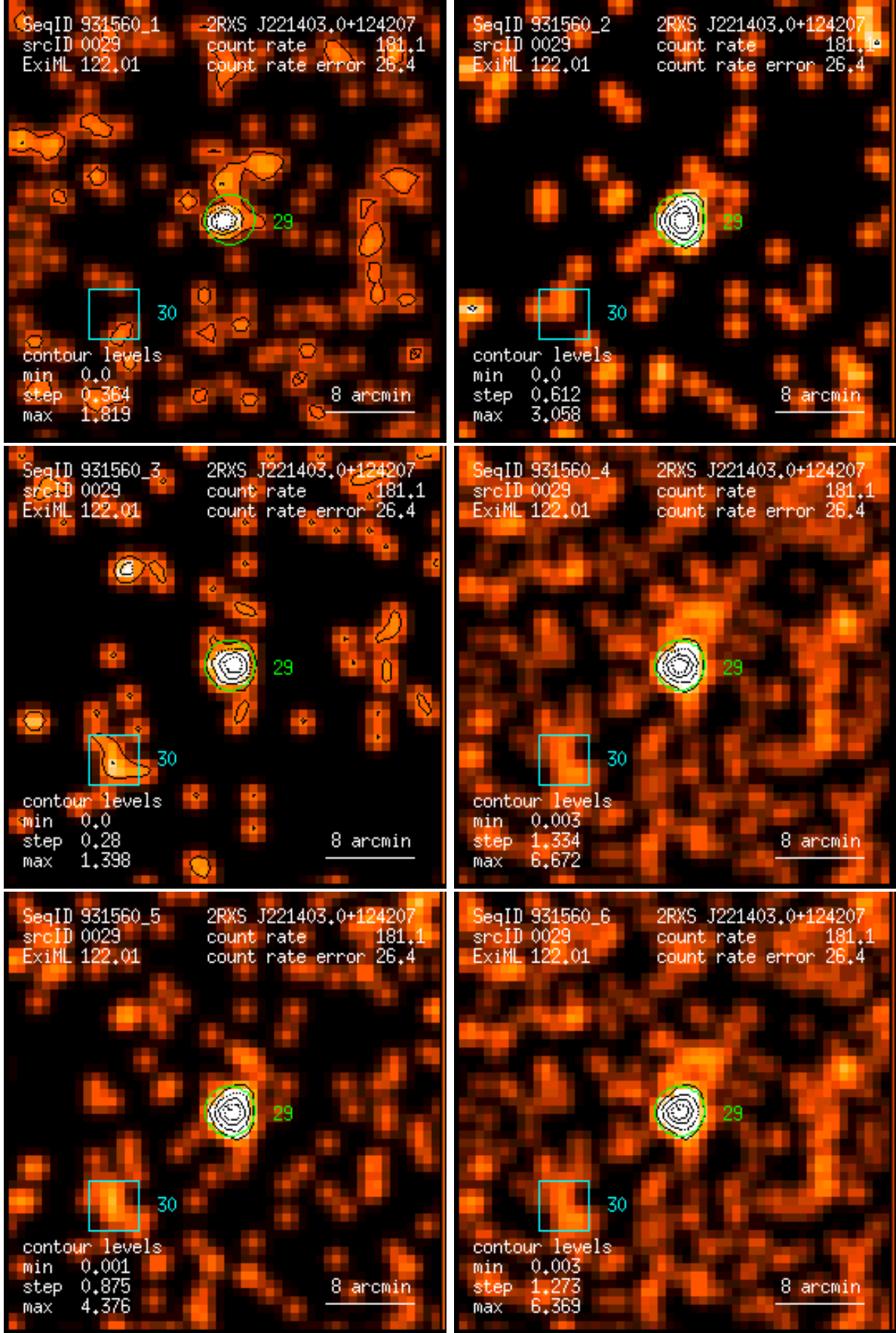
Figure 29: RASS 931560: detection 0029: band rate images, Gaussian filter: (1) PSPC channels 11 – 41, (2) 52 – 90, (3) 91 – 201, (4) 11 – 235, (5) 52 – 201, (6) 11 – 201. Broad band rates in counts/ks. Band rate contour levels in counts/ks/arcmin 2 .
