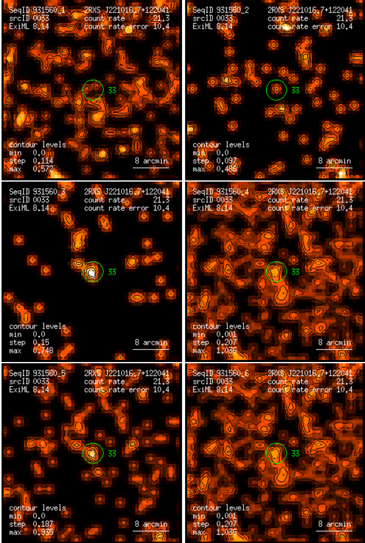
Figure 33: RASS 931560: detection 0033: band rate images, Gaussian filter: (1) PSPC channels 11 – 41, (2) 52 – 90, (3) 91 – 201, (4) 11 – 235, (5) 52 – 201, (6) 11 – 201. Broad band rates in counts/ks. Band rate contour levels in counts/ks/arcmin 2 .
