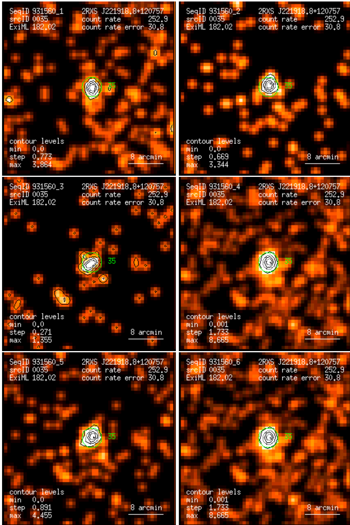
Figure 35: RASS 931560: detection 0035: band rate images, Gaussian filter: (1) PSPC channels 11 – 41, (2) 52 – 90, (3) 91 – 201, (4) 11 – 235, (5) 52 – 201, (6) 11 – 201. Broad band rates in counts/ks. Band rate contour levels in counts/ks/arcmin 2 .
