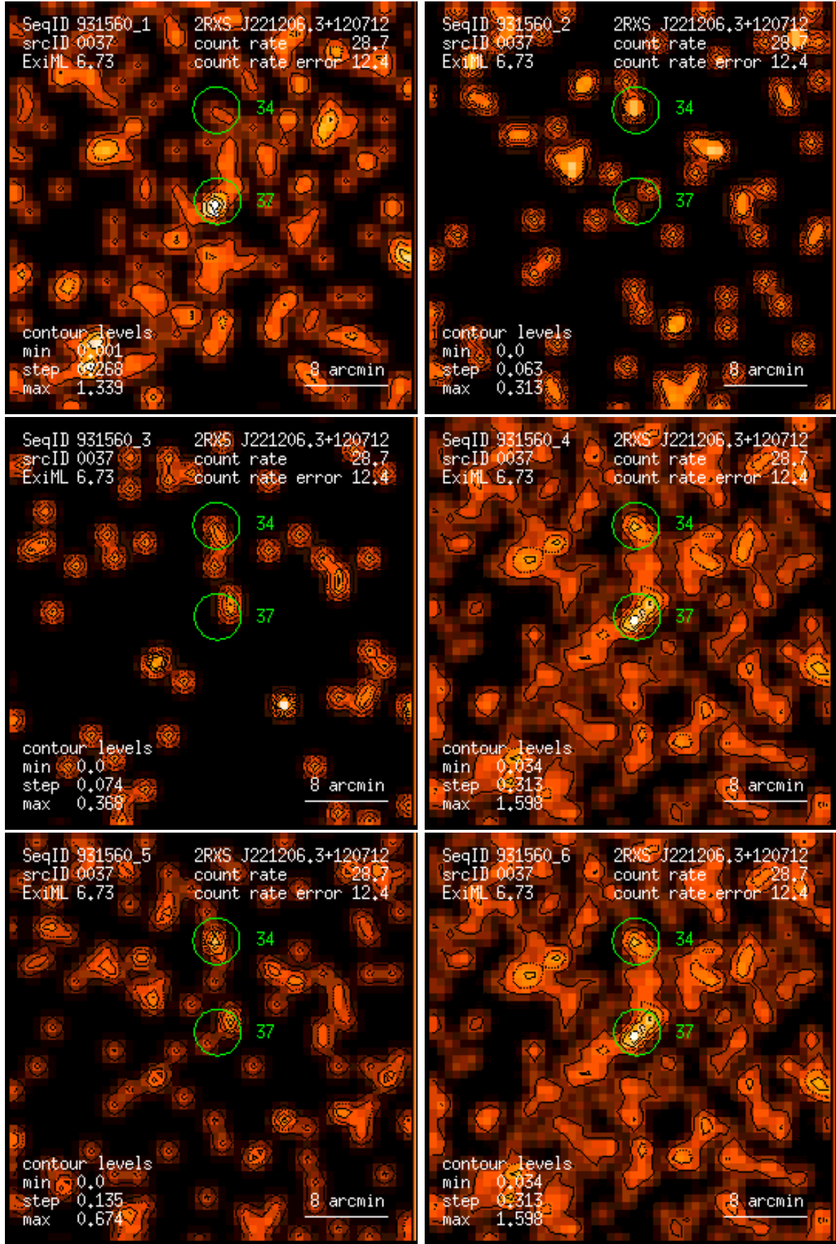
Figure 37: RASS 931560: detection 0037: band rate images, Gaussian filter: (1) PSPC channels 11 – 41, (2) 52 – 90, (3) 91 – 201, (4) 11 – 235, (5) 52 – 201, (6) 11 – 201. Broad band rates in counts/ks. Band rate contour levels in counts/ks/arcmin 2 .
