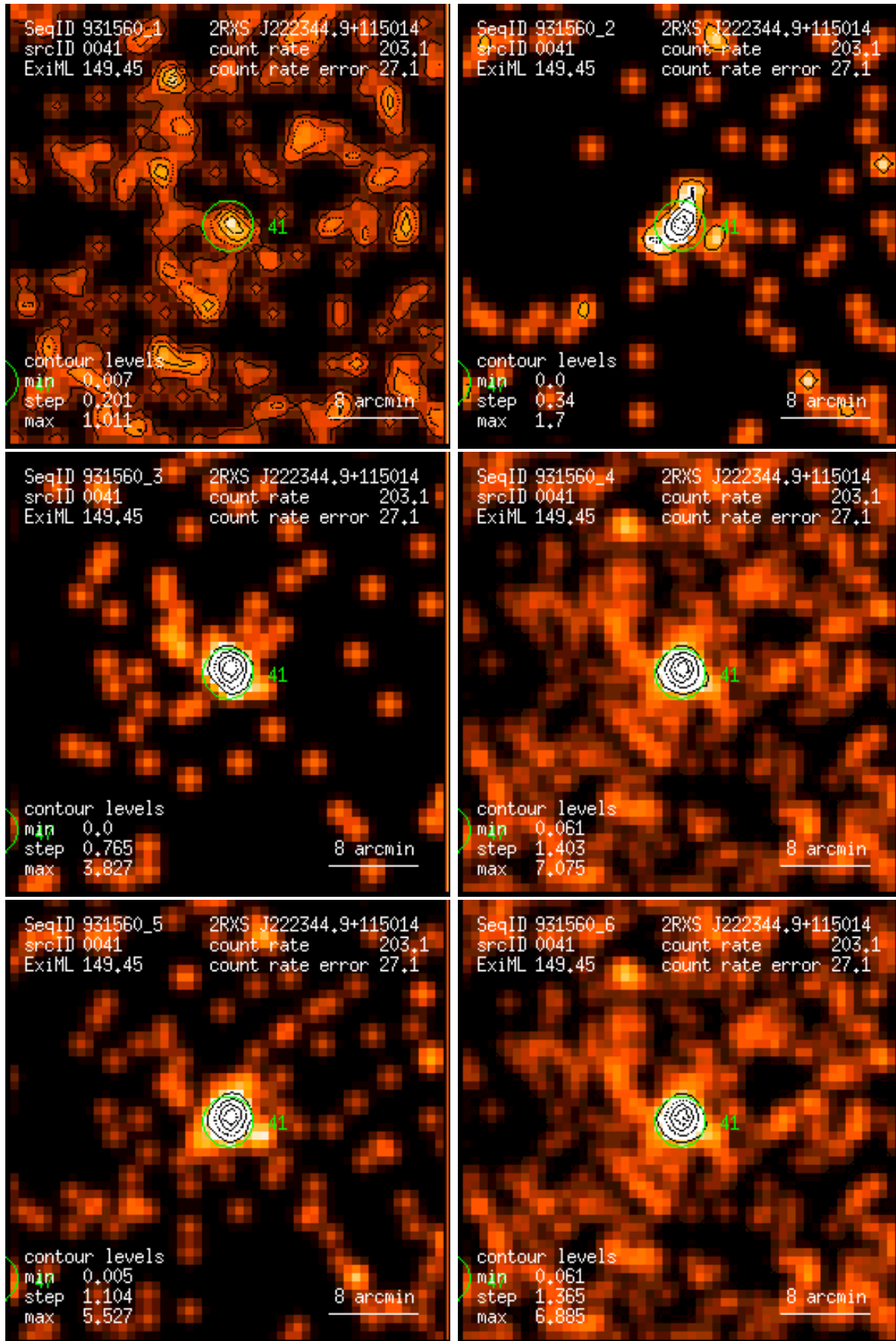
Figure 41: RASS 931560: detection 0041: band rate images, Gaussian filter: (1) PSPC channels 11 – 41, (2) 52 – 90, (3) 91 – 201, (4) 11 – 235, (5) 52 – 201, (6) 11 – 201. Broad band rates in counts/ks. Band rate contour levels in counts/ks/arcmin 2 .
