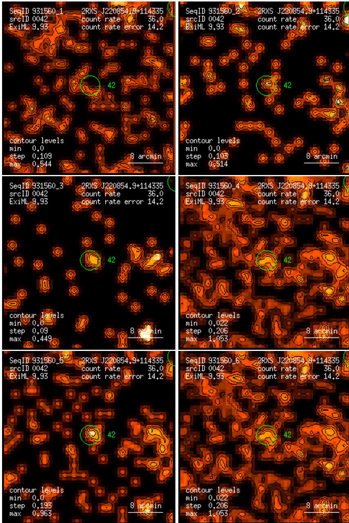
Figure 42: RASS 931560: detection 0042: band rate images, Gaussian filter: (1) PSPC channels 11 – 41, (2) 52 – 90, (3) 91 – 201, (4) 11 – 235, (5) 52 – 201, (6) 11 – 201. Broad band rates in counts/ks. Band rate contour levels in counts/ks/arcmin 2 .
