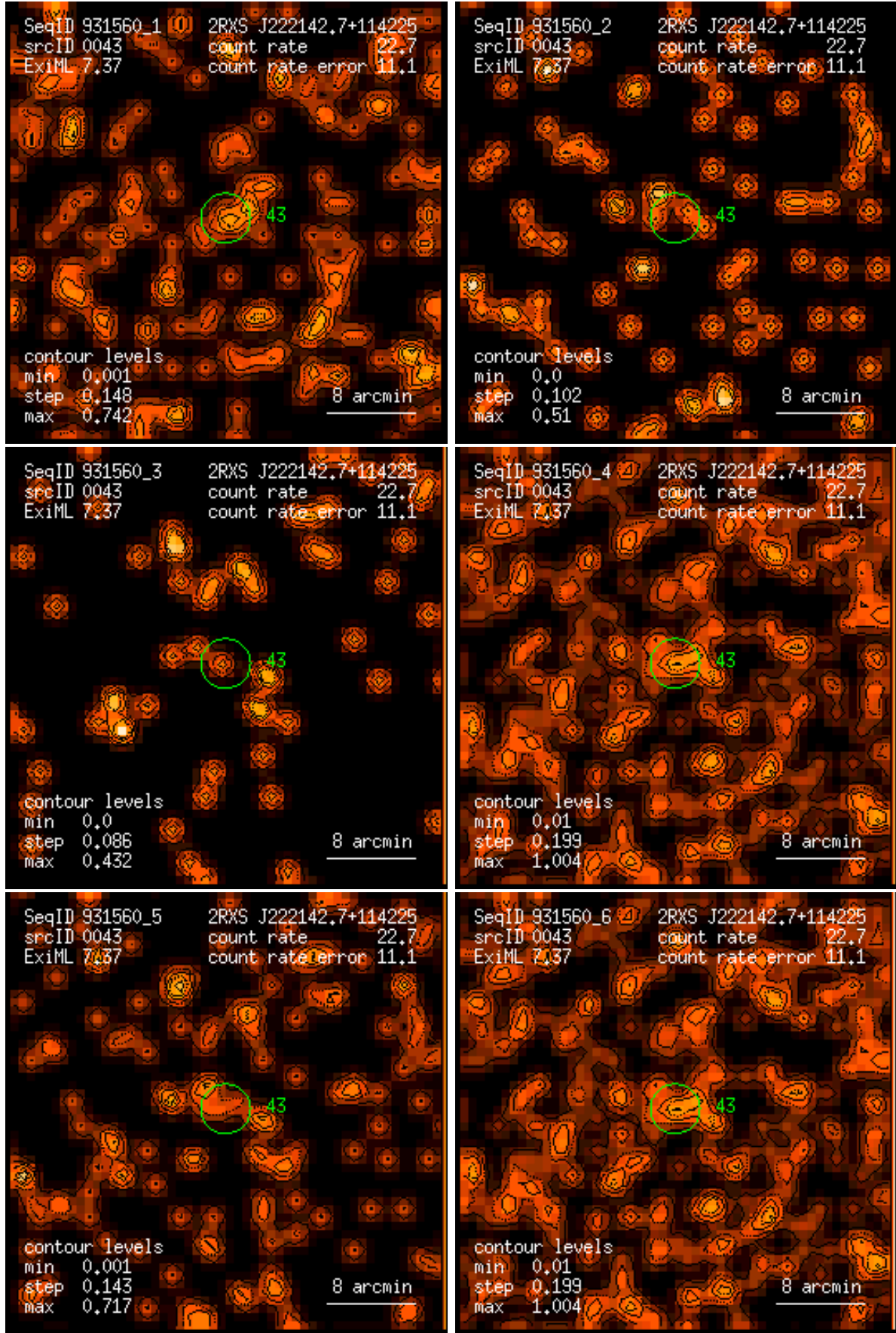
Figure 43: RASS 931560: detection 0043: band rate images, Gaussian filter: (1) PSPC channels 11 – 41, (2) 52 – 90, (3) 91 – 201, (4) 11 – 235, (5) 52 – 201, (6) 11 – 201. Broad band rates in counts/ks. Band rate contour levels in counts/ks/arcmin 2 .
