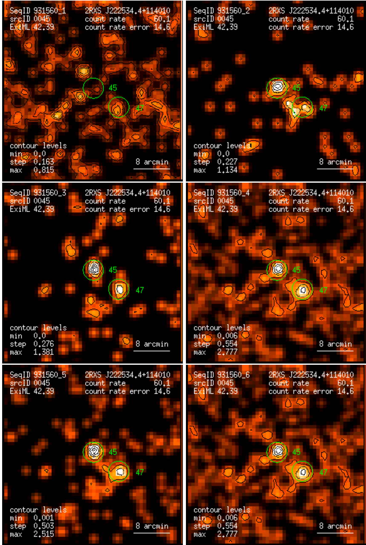
Figure 45: RASS 931560: detection 0045: band rate images, Gaussian filter: (1) PSPC channels 11 – 41, (2) 52 – 90, (3) 91 – 201, (4) 11 – 235, (5) 52 – 201, (6) 11 – 201. Broad band rates in counts/ks. Band rate contour levels in counts/ks/arcmin 2 .
