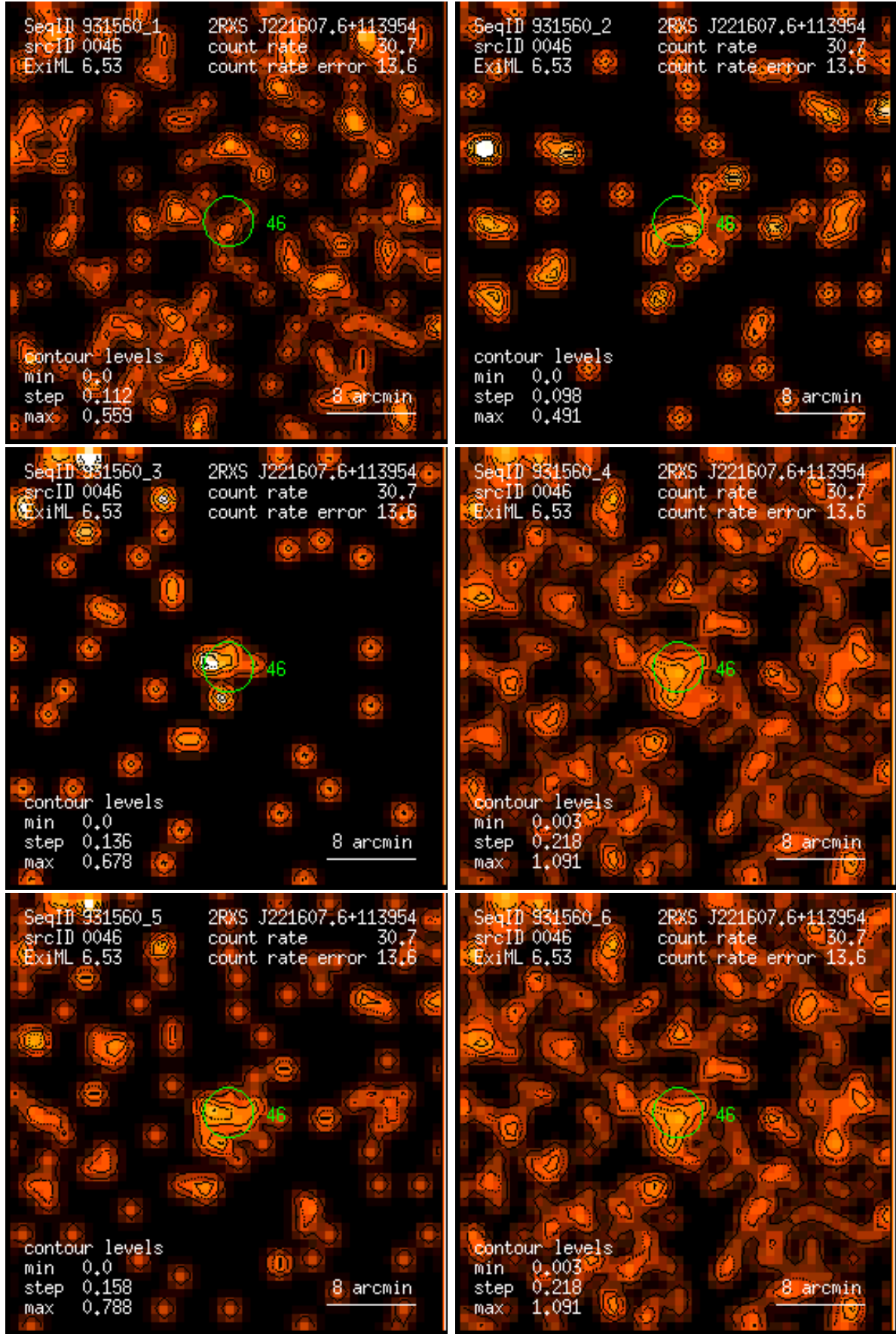
Figure 46: RASS 931560: detection 0046: band rate images, Gaussian filter: (1) PSPC channels 11 – 41, (2) 52 – 90, (3) 91 – 201, (4) 11 – 235, (5) 52 – 201, (6) 11 – 201. Broad band rates in counts/ks. Band rate contour levels in counts/ks/arcmin 2 .
