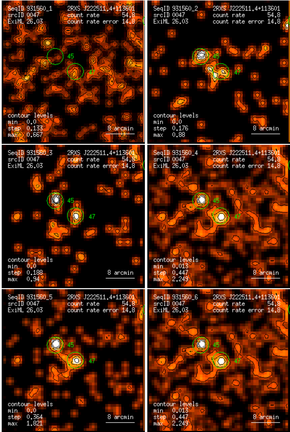
Figure 47: RASS 931560: detection 0047: band rate images, Gaussian filter: (1) PSPC channels 11 – 41, (2) 52 – 90, (3) 91 – 201, (4) 11 – 235, (5) 52 – 201, (6) 11 – 201. Broad band rates in counts/ks. Band rate contour levels in counts/ks/arcmin 2 .
