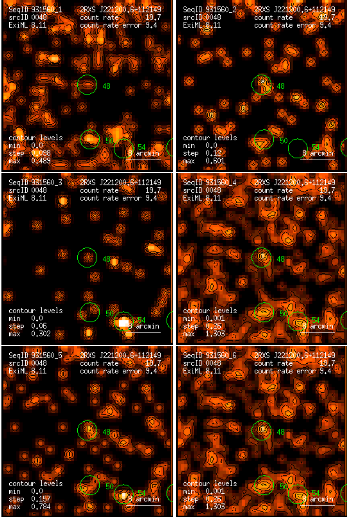
Figure 48: RASS 931560: detection 0048: band rate images, Gaussian filter: (1) PSPC channels 11 – 41, (2) 52 – 90, (3) 91 – 201, (4) 11 – 235, (5) 52 – 201, (6) 11 – 201. Broad band rates in counts/ks. Band rate contour levels in counts/ks/arcmin 2 .
