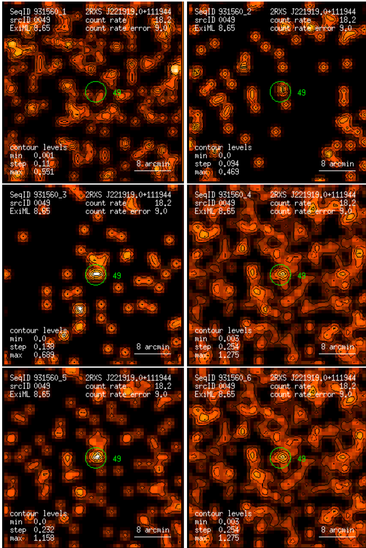
Figure 49: RASS 931560: detection 0049: band rate images, Gaussian filter: (1) PSPC channels 11 – 41, (2) 52 – 90, (3) 91 – 201, (4) 11 – 235, (5) 52 – 201, (6) 11 – 201. Broad band rates in counts/ks. Band rate contour levels in counts/ks/arcmin 2 .
