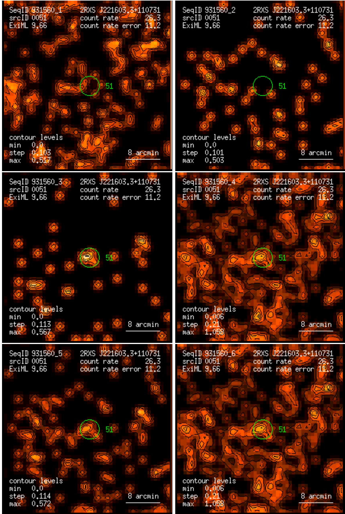
Figure 51: RASS 931560: detection 0051: band rate images, Gaussian filter: (1) PSPPC channels 11 – 41, (2) 52 – 90, (3) 91 – 201, (4) 11 – 235, (5) 52 – 201, (6) 11 – 201. Broad band rates in counts/ks. Band rate contour levels in counts/ks/arcmin 2 .
