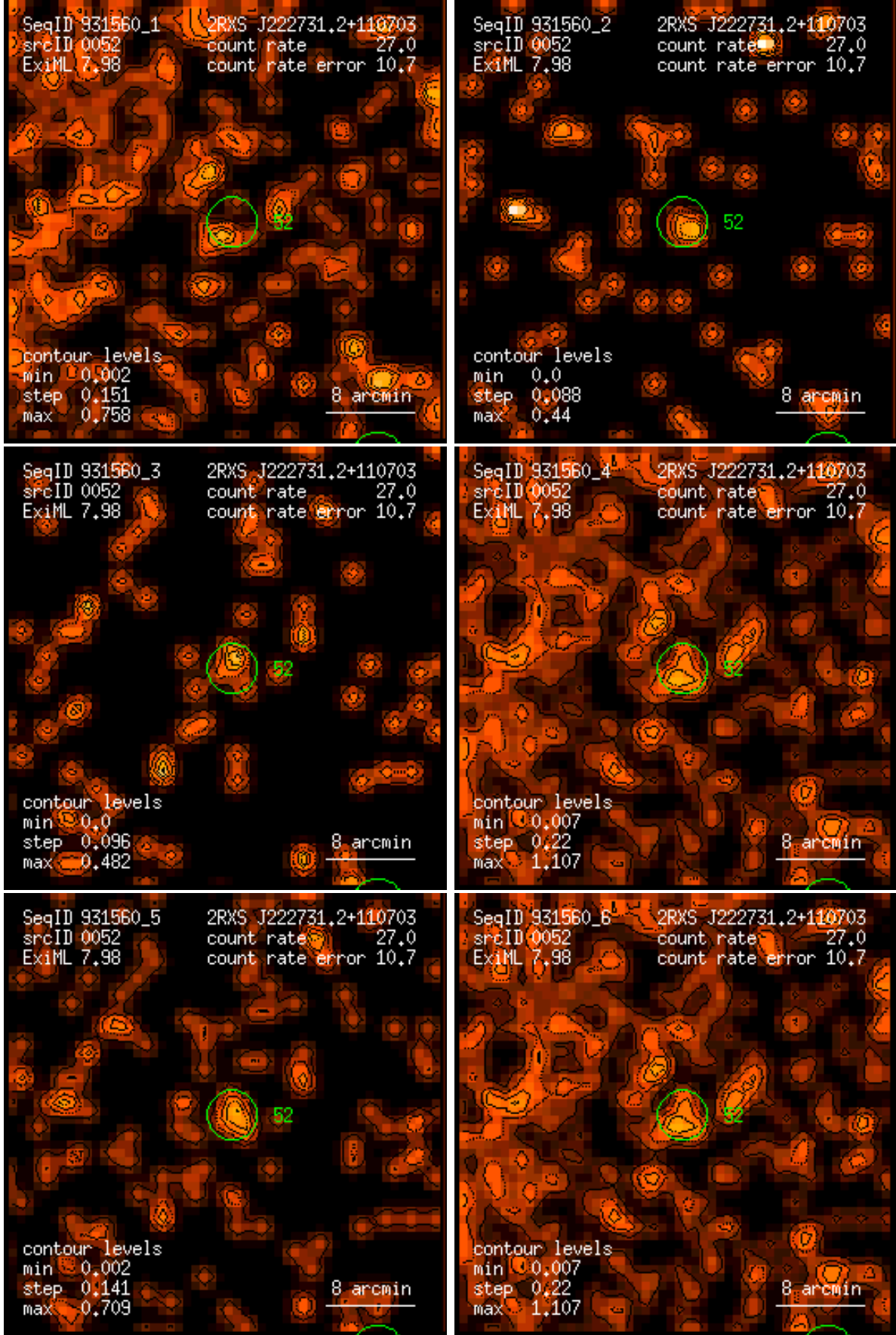
Figure 52: RASS 931560: detection 0052: band rate images, Gaussian filter: (1) PSPC channels 11 – 41, (2) 52 – 90, (3) 91 – 201, (4) 11 – 235, (5) 52 – 201, (6) 11 – 201. Broad band rates in counts/ks. Band rate contour levels in counts/ks/arcmin 2 .
