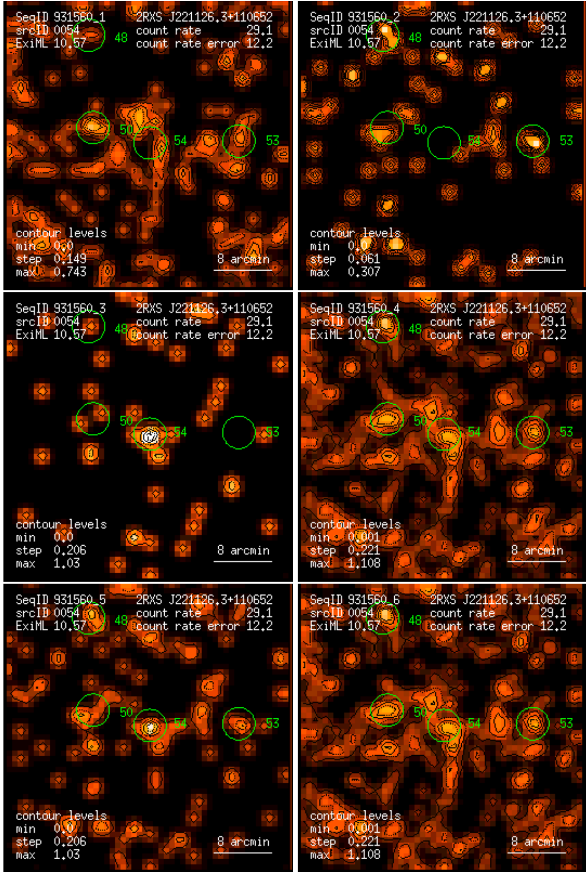
Figure 54: RASS 931560: detection 0054: band rate images, Gaussian filter: (1) PSPC channels 11 – 41, (2) 52 – 90, (3) 91 – 201, (4) 11 – 235, (5) 52 – 201, (6) 11 – 201. Broad band rates in counts/ks. Band rate contour levels in counts/ks/arcmin 2 .
