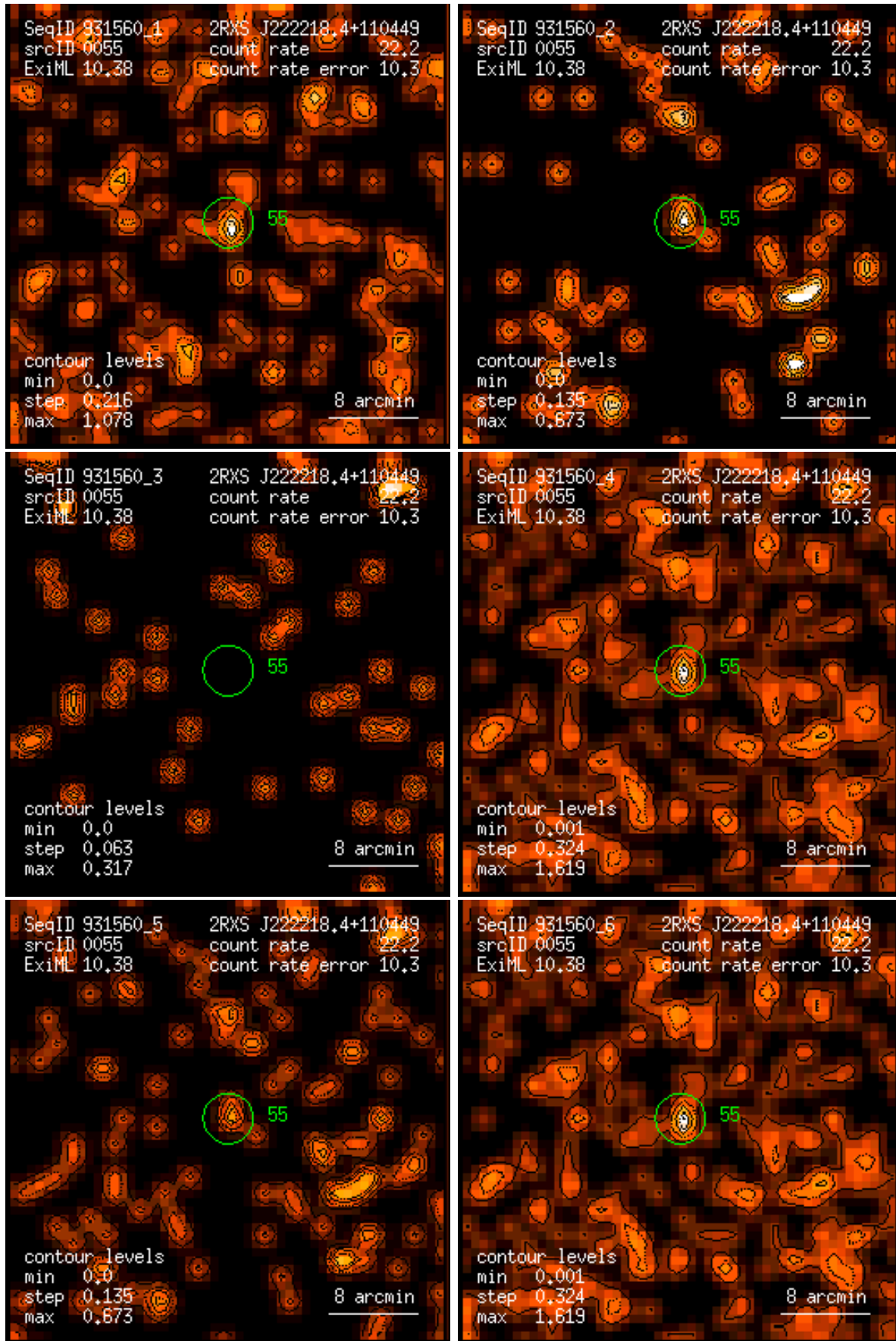
Figure 55: RASS 931560: detection 0055: band rate images, Gaussian filter: (1) PSPC channels 11 – 41, (2) 52 – 90, (3) 91 – 201, (4) 11 – 235, (5) 52 – 201, (6) 11 – 201. Broad band rates in counts/ks. Band rate contour levels in counts/ks/arcmin 2 .
