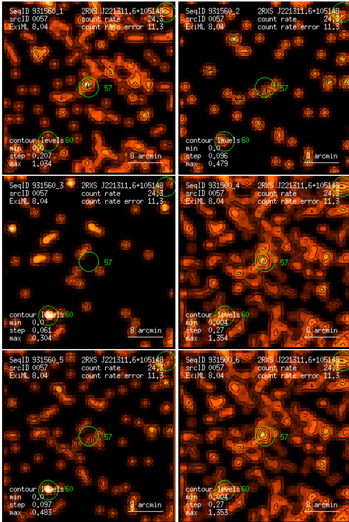
Figure 57: RASS 931560: detection 0057: band rate images, Gaussian filter: (1) PSPC channels 11 – 41, (2) 52 – 90, (3) 91 – 201, (4) 11 – 235, (5) 52 – 201, (6) 11 – 201. Broad band rates in counts/ks. Band rate contour levels in counts/ks/arcmin 2 .
