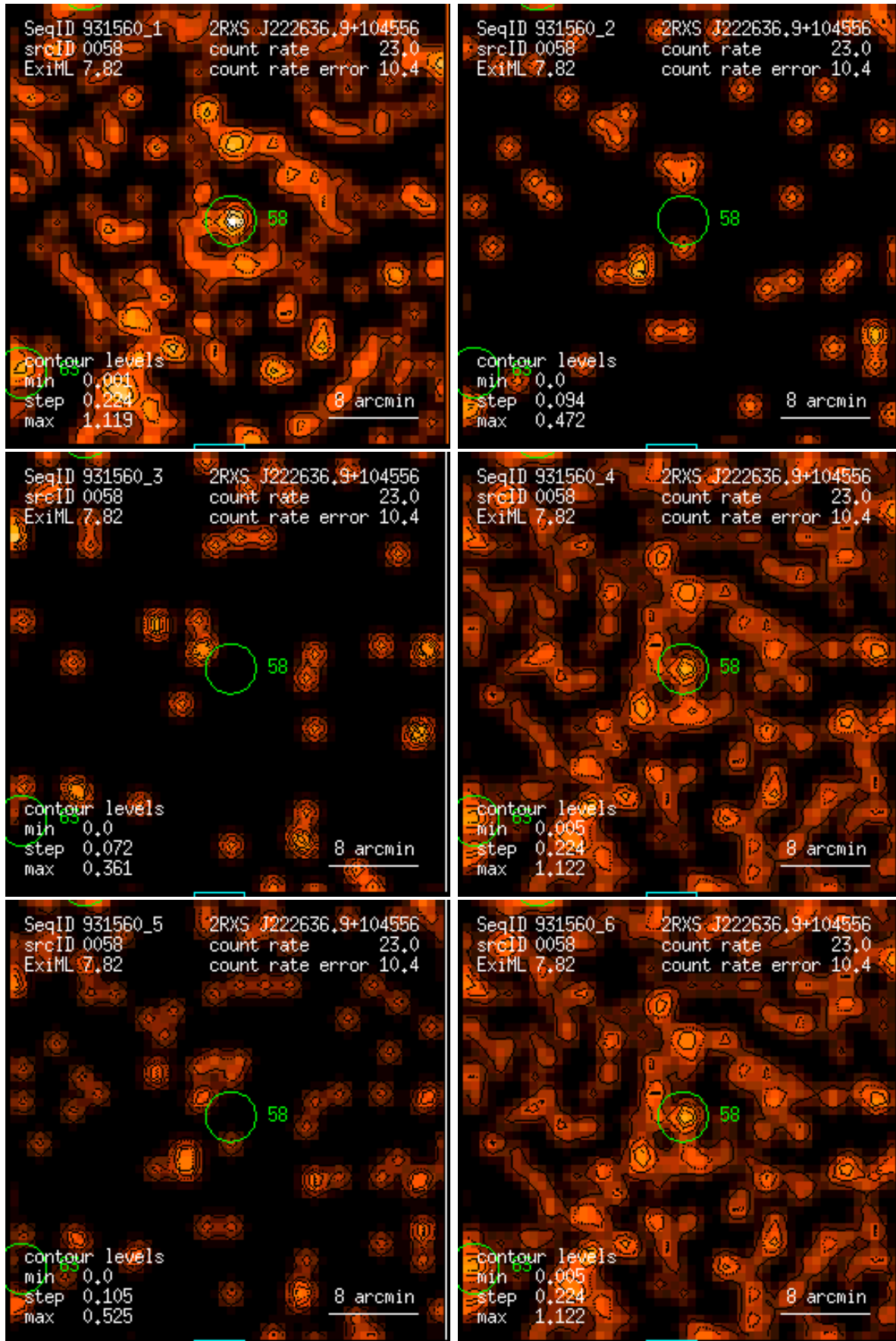
Figure 58: RASS 931560: detection 0058: band rate images, Gaussian filter: (1) PSPC channels 11 – 41, (2) 52 – 90, (3) 91 – 201, (4) 11 – 235, (5) 52 – 201, (6) 11 – 201. Broad band rates in counts/ks. Band rate contour levels in counts/ks/arcmin 2 .
