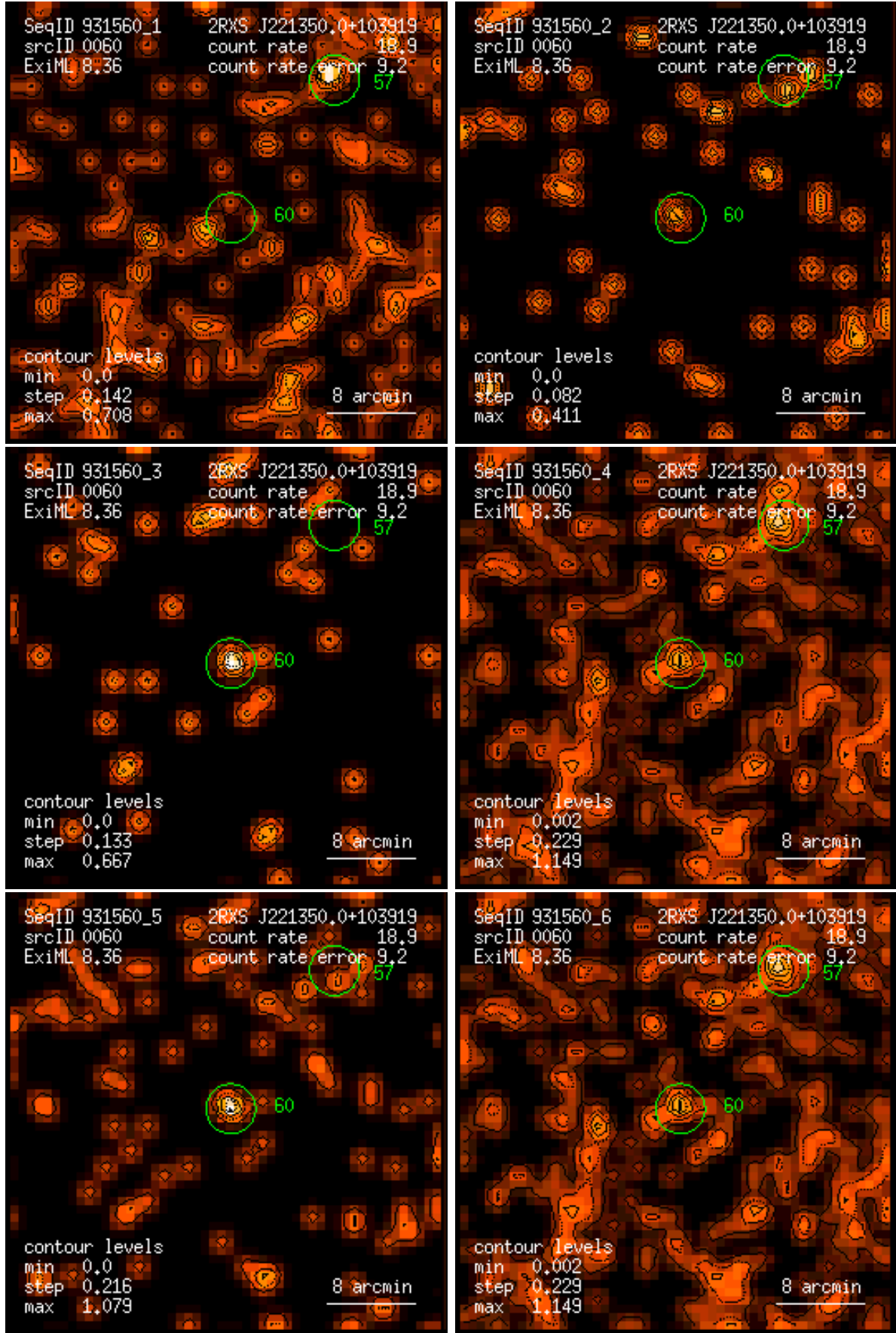
Figure 60: RASS 931560: detection 0060: band rate images, Gaussian filter: (1) PSPC channels 11 – 41, (2) 52 – 90, (3) 91 – 201, (4) 11 – 235, (5) 52 – 201, (6) 11 – 201. Broad band rates in counts/ks. Band rate contour levels in counts/ks/arcmin 2 .
