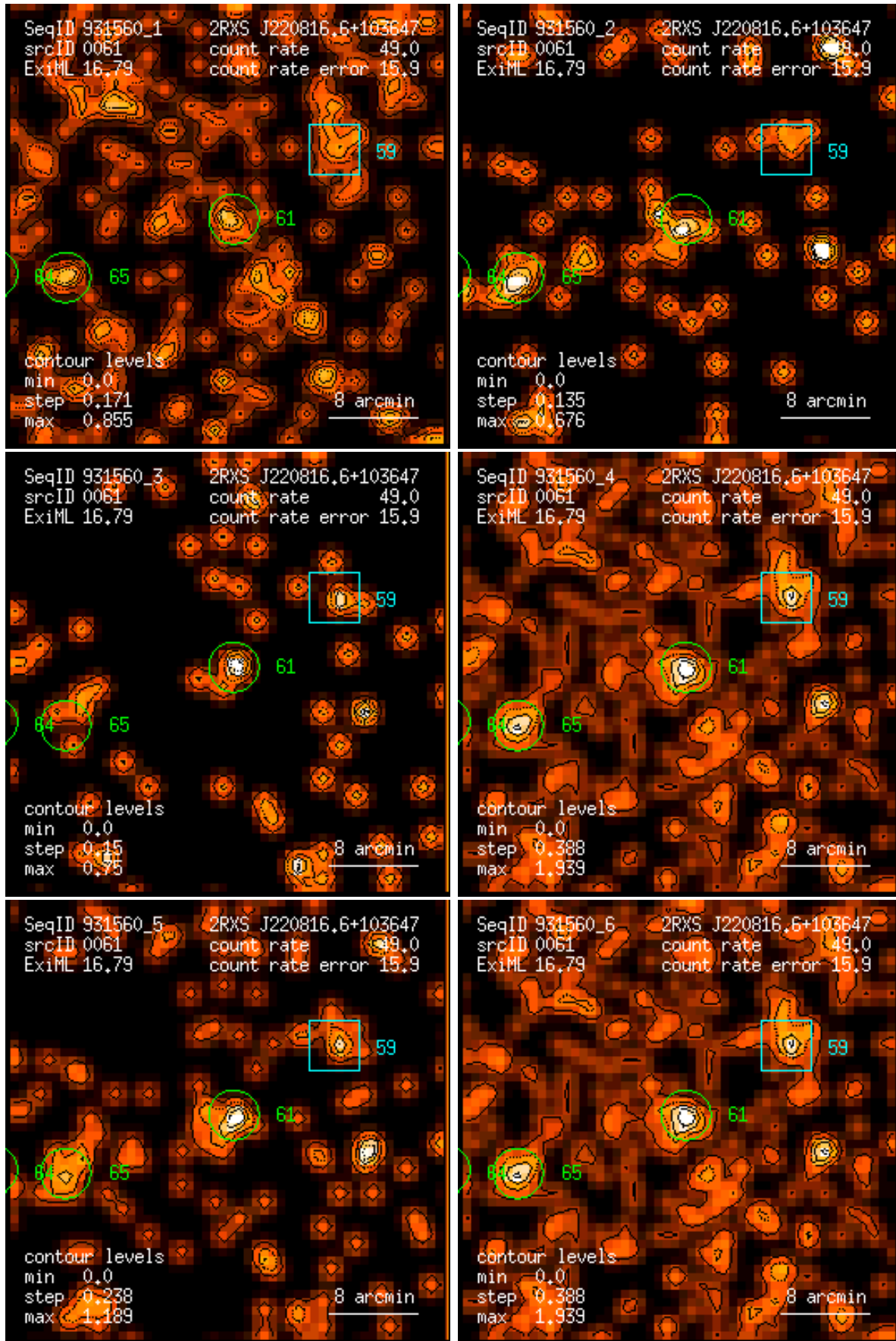
Figure 61: RASS 931560: detection 0061: band rate images, Gaussian filter: (1) PSPC channels 11 – 41, (2) 52 – 90, (3) 91 – 201, (4) 11 – 235, (5) 52 – 201, (6) 11 – 201. Broad band rates in counts/ks. Band rate contour levels in counts/ks/arcmin 2 .
