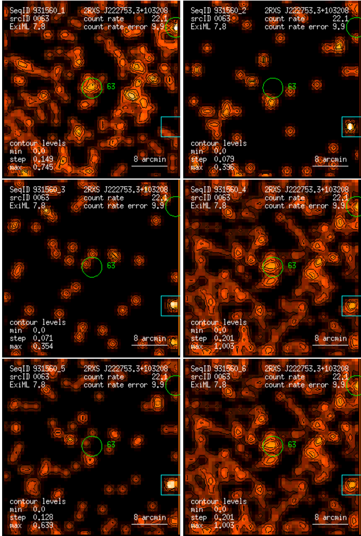
Figure 63: RASS 931560: detection 0063: band rate images, Gaussian filter: (1) PSPC channels 11 – 41, (2) 52 – 90, (3) 91 – 201, (4) 11 – 235, (5) 52 – 201, (6) 11 – 201. Broad band rates in counts/ks. Band rate contour levels in counts/ks/arcmin 2 .
