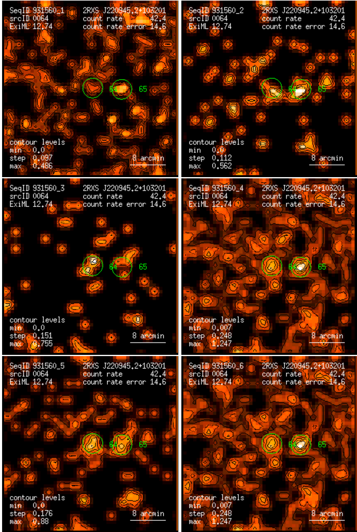
Figure 64: RASS 931560: detection 0064: band rate images, Gaussian filter: (1) PSPC channels 11 – 41, (2) 52 – 90, (3) 91 – 201, (4) 11 – 235, (5) 52 – 201, (6) 11 – 201. Broad band rates in counts/ks. Band rate contour levels in counts/ks/arcmin 2 .
