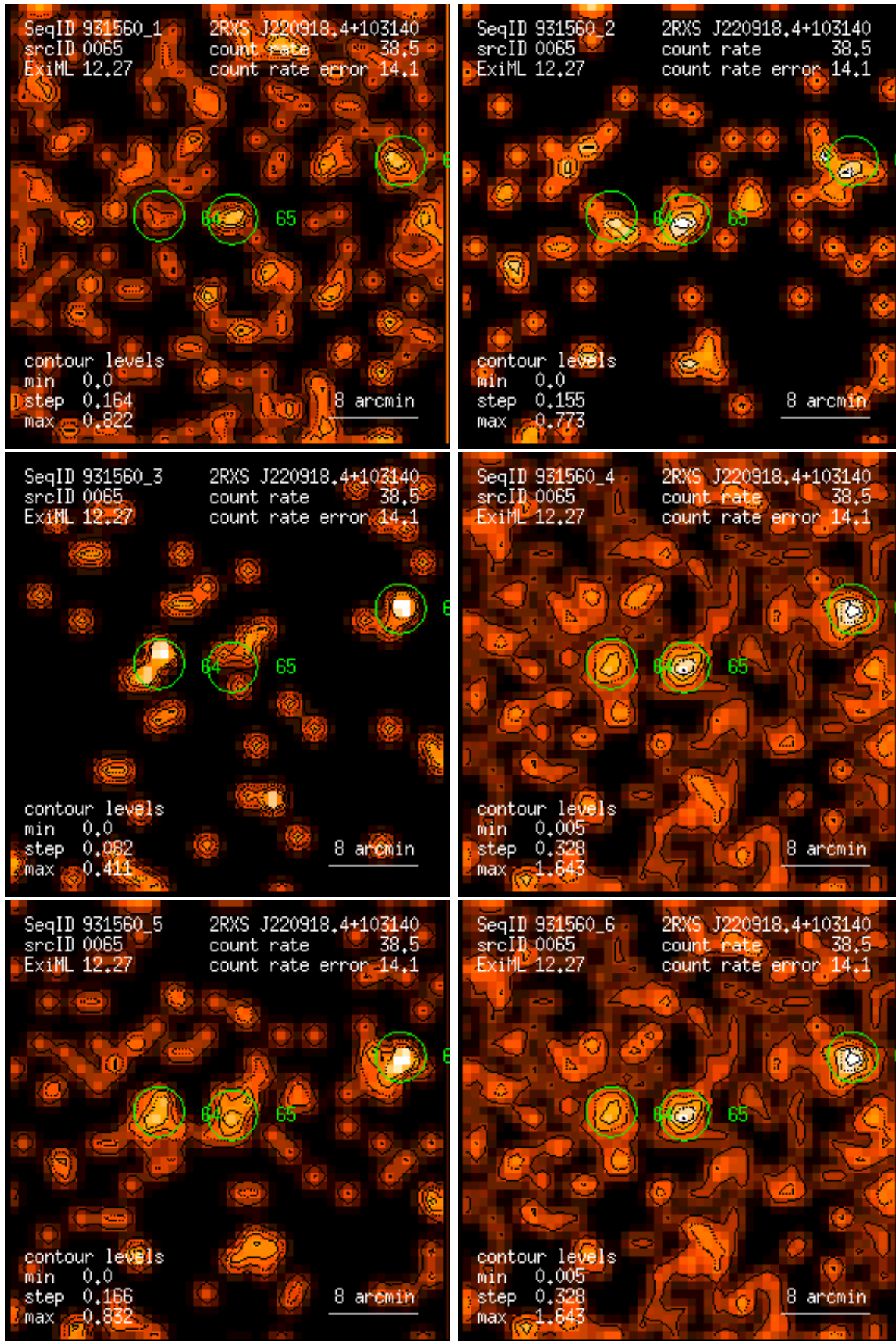
Figure 65: RASS 931560: detection 0065: band rate images, Gaussian filter: (1) PSPC channels 11 – 41, (2) 52 – 90, (3) 91 – 201, (4) 11 – 235, (5) 52 – 201, (6) 11 – 201. Broad band rates in counts/ks. Band rate contour levels in counts/ks/arcmin 2 .
