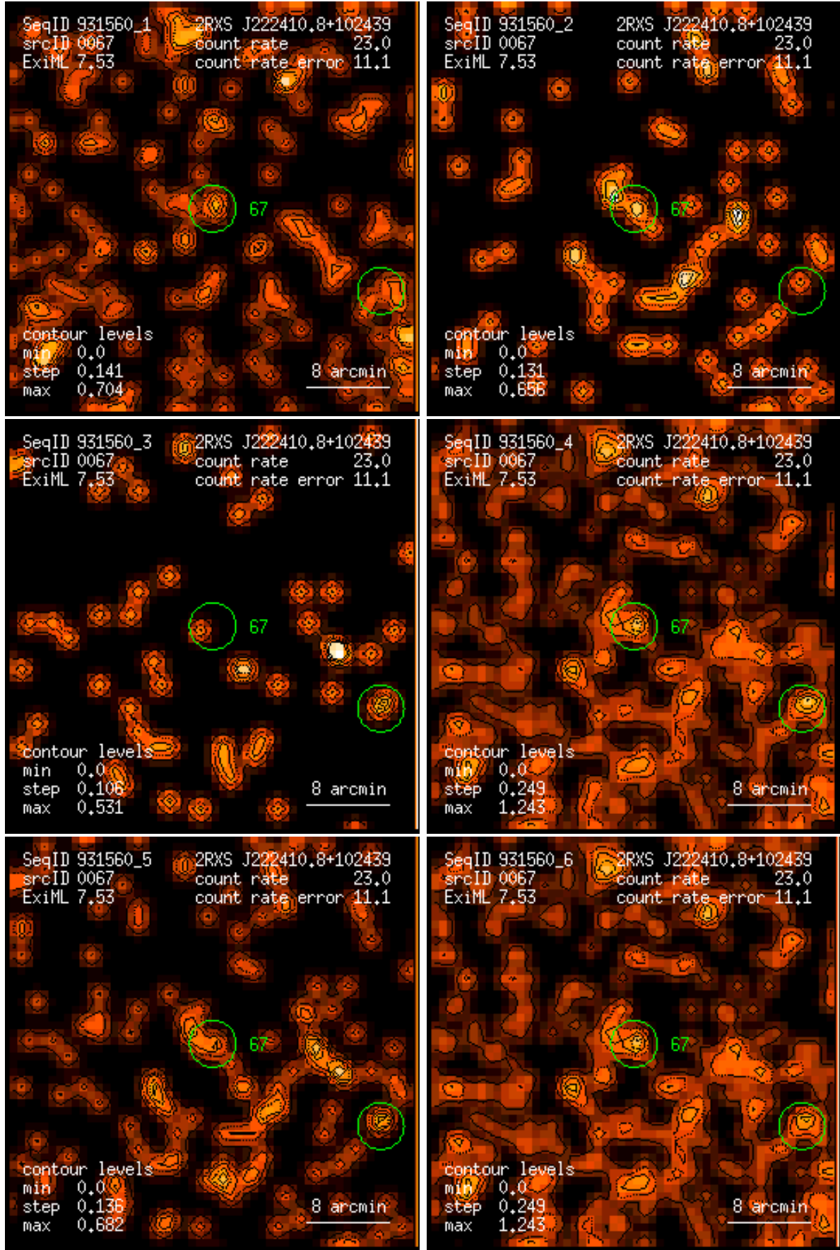
Figure 67: RASS 931560: detection 0067: band rate images, Gaussian filter: (1) PSPC channels 11 – 41, (2) 52 – 90, (3) 91 – 201, (4) 11 – 235, (5) 52 – 201, (6) 11 – 201. Broad band rates in counts/ks. Band rate contour levels in counts/ks/arcmin 2 .
