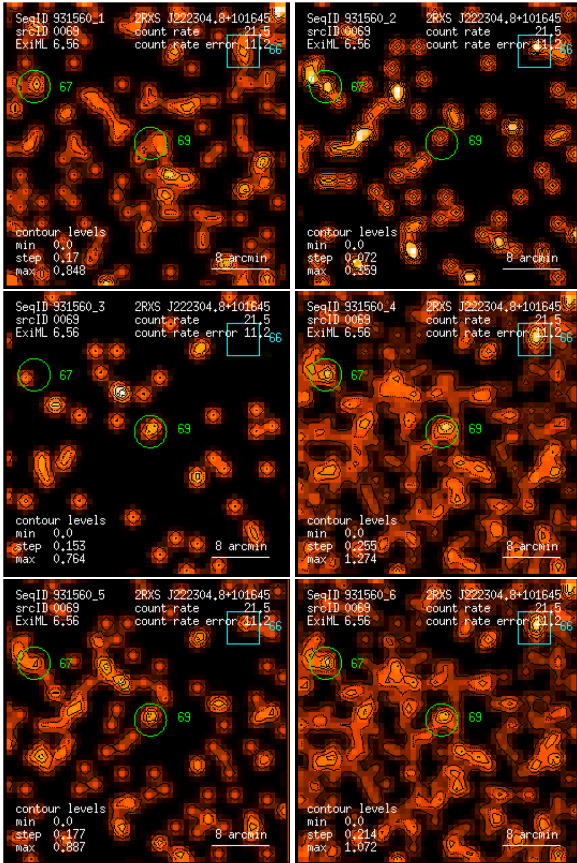
Figure 69: RASS 931560: detection 0069: band rate images, Gaussian filter: (1) PSPC channels 11 – 41, (2) 52 – 90, (3) 91 – 201, (4) 11 – 235, (5) 52 – 201, (6) 11 – 201. Broad band rates in counts/ks. Band rate contour levels in counts/ks/arcmin 2 .
