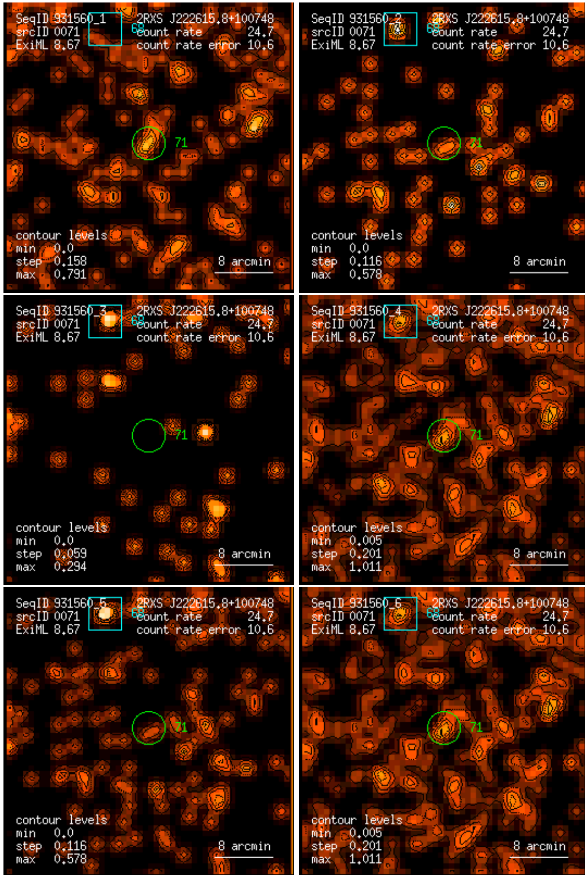
Figure 71: RASS 931560: detection 0071: band rate images, Gaussian filter: (1) PSPC channels 11 – 41, (2) 52 – 90, (3) 91 – 201, (4) 11 – 235, (5) 52 – 201, (6) 11 – 201. Broad band rates in counts/ks. Band rate contour levels in counts/ks/arcmin 2 .
