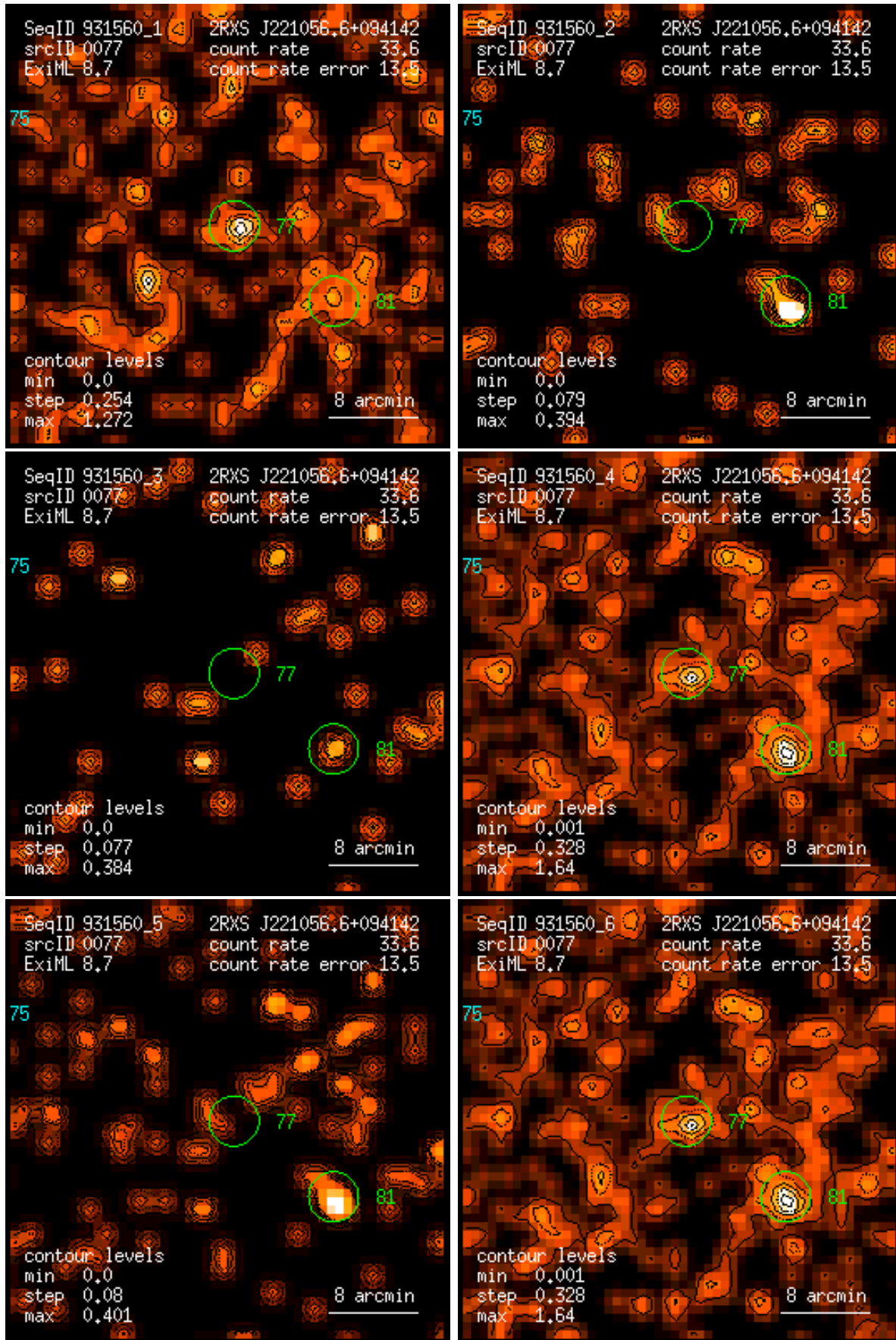
Figure 77: RASS 931560: detection 0077: band rate images, Gaussian filter: (1) PSPC channels 11 – 41, (2) 52 – 90, (3) 91 – 201, (4) 11 – 235, (5) 52 – 201, (6) 11 – 201. Broad band rates in counts/ks. Band rate contour levels in counts/ks/arcmin 2 .
