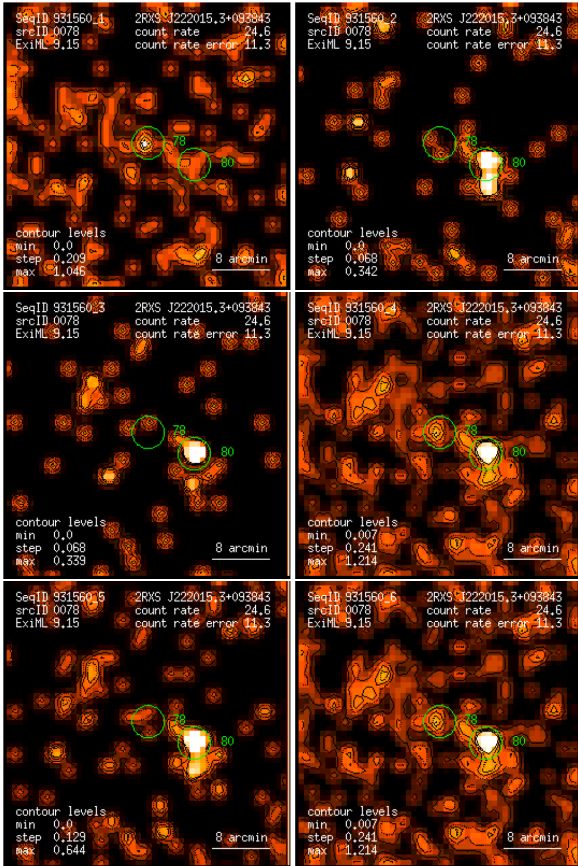
Figure 78: RASS 931560: detection 0078: band rate images, Gaussian filter: (1) PSPC channels 11 – 41, (2) 52 – 90, (3) 91 – 201, (4) 11 – 235, (5) 52 – 201, (6) 11 – 201. Broad band rates in counts/ks. Band rate contour levels in counts/ks/arcmin 2 .
