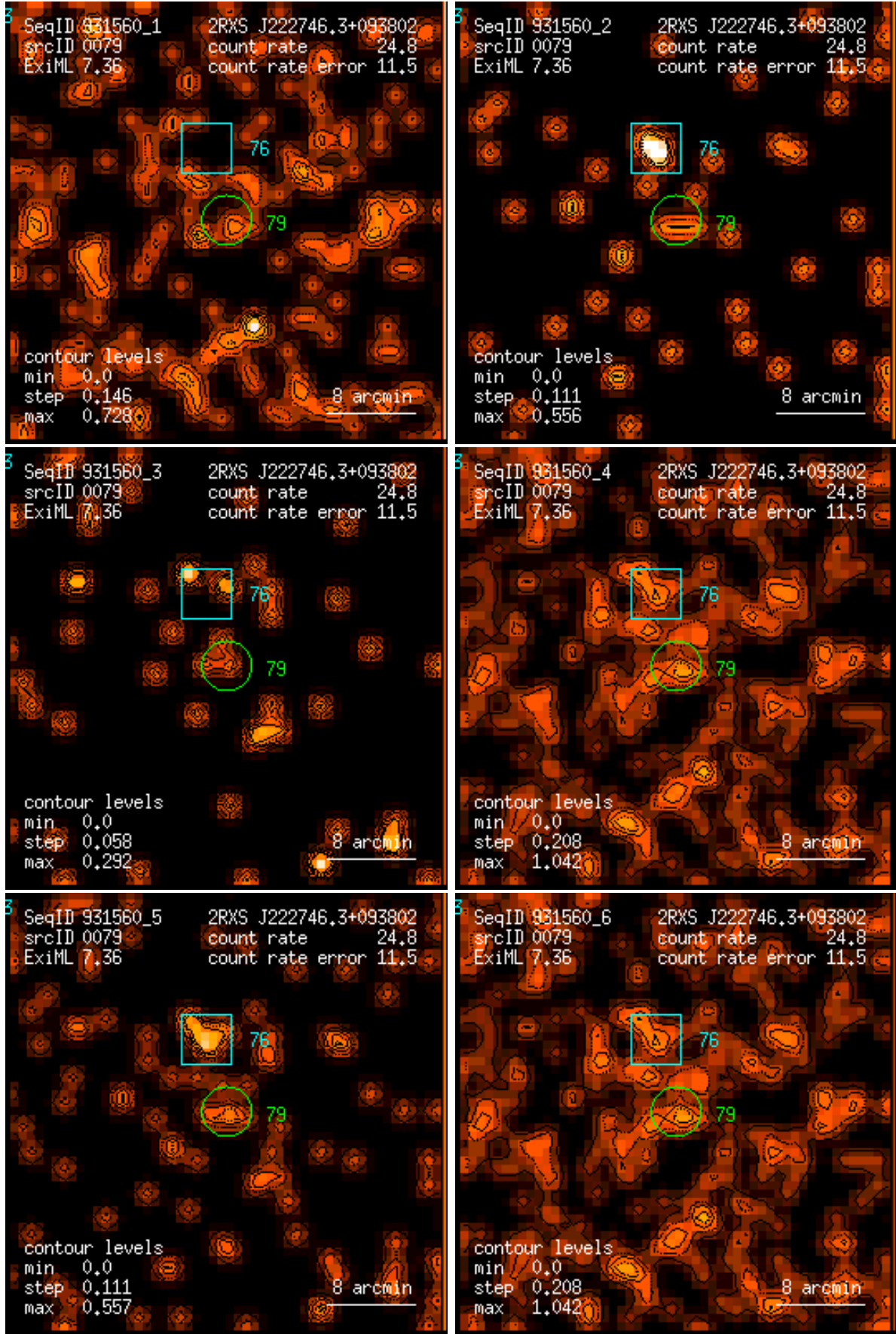
Figure 79: RASS 931560: detection 0079: band rate images, Gaussian filter: (1) PSPC channels 11 – 41, (2) 52 – 90, (3) 91 – 201, (4) 11 – 235, (5) 52 – 201, (6) 11 – 201. Broad band rates in counts/ks. Band rate contour levels in counts/ks/arcmin 2 .
